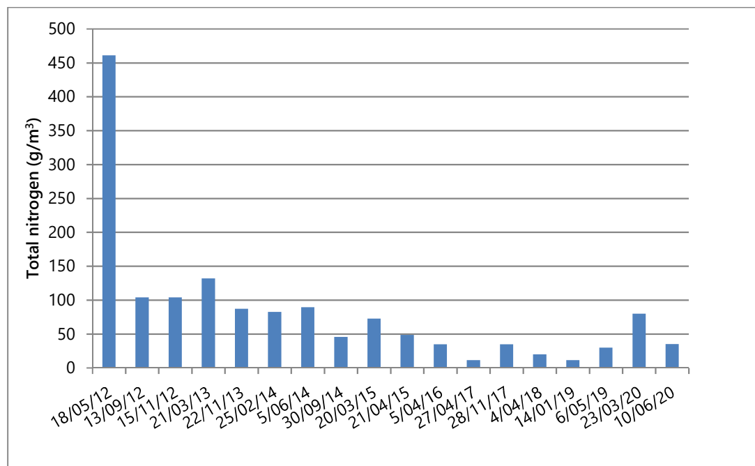
Figure 2 Concentrations of total nitrogen in the irrigated wastewater
