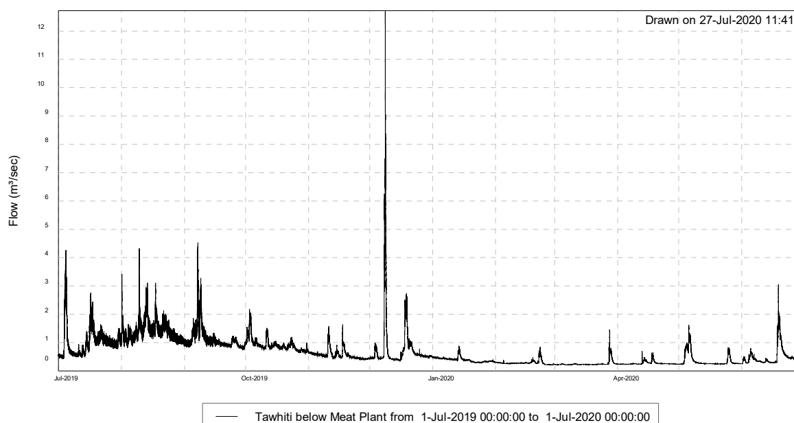
Figure 4 Flow ( \text{m}^3/\text{s} ) in the Tawhiti Stream measured below the abstraction point of Silver Fern Farms from 1 July 2019 to 30 June 2020
