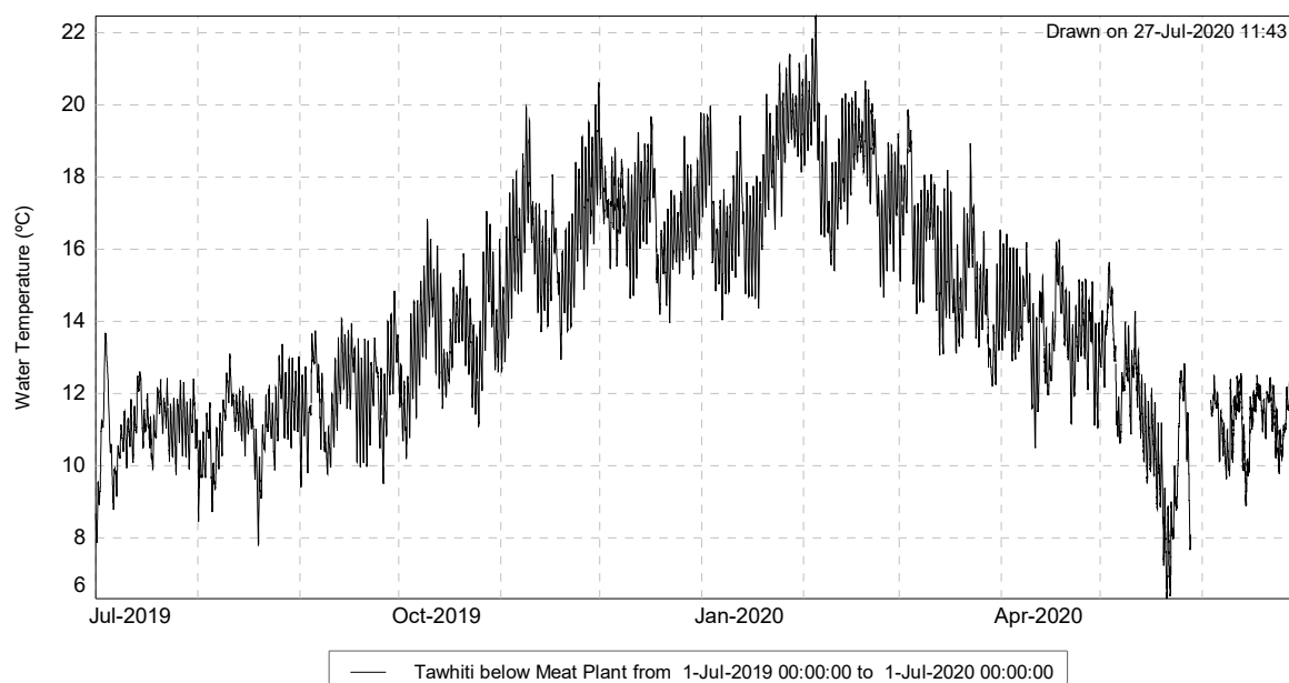
Figure 5 Temperature of Tawhiti Stream at Tawhiti Road, July 2019 – June 2020, °C
