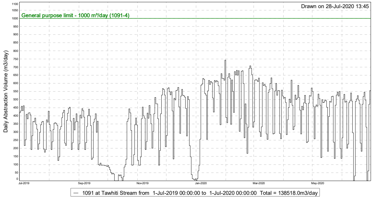
Figure 2 Daily water abstraction by Silver Fern Farms, July 2019-June 2020, m 3
