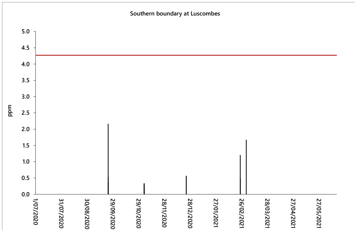
Figure 16 Atmospheric ammonia concentration at ground level on the site boundary (consent limit 4.27 ppm one hour average)
