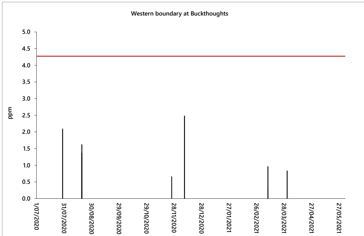
Figure 15 Atmospheric ammonia concentration at ground level on the site boundary (consent limit 4.27 ppm one hour average)
