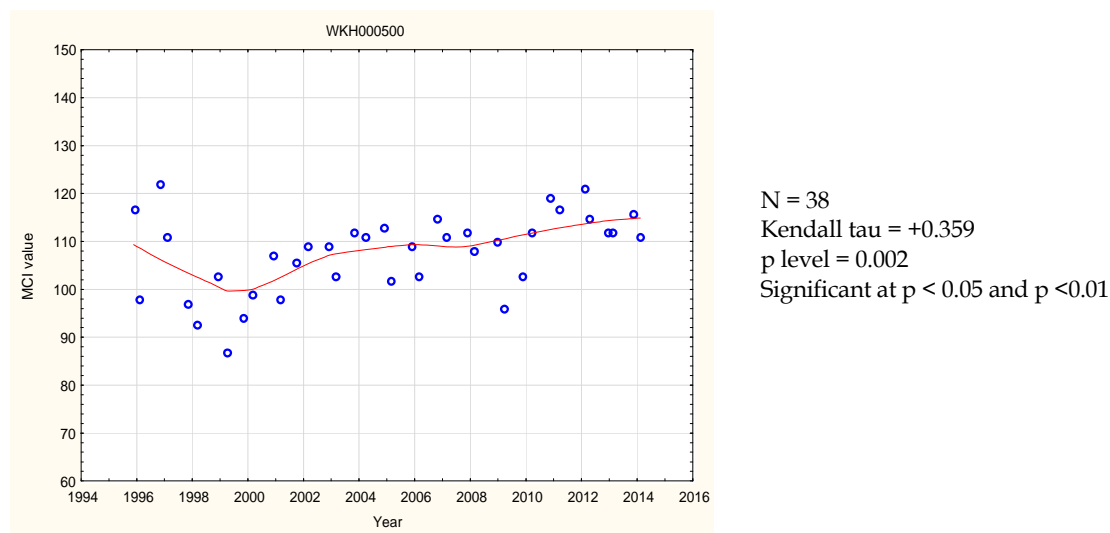
Figure 19 LOWESS trend plot at the Egmont Village site
