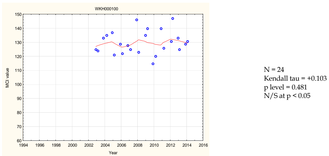
Figure 17 LOWESS trend plot of MCI data at the National Park site
