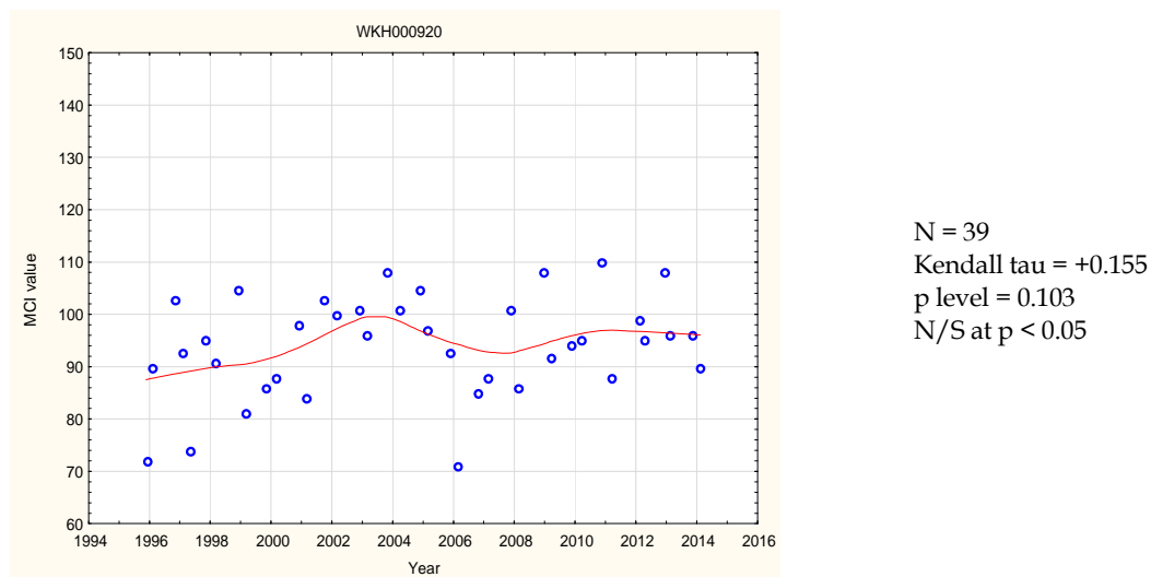
Figure 21 LOWESS trend plot at the Constance Street site
