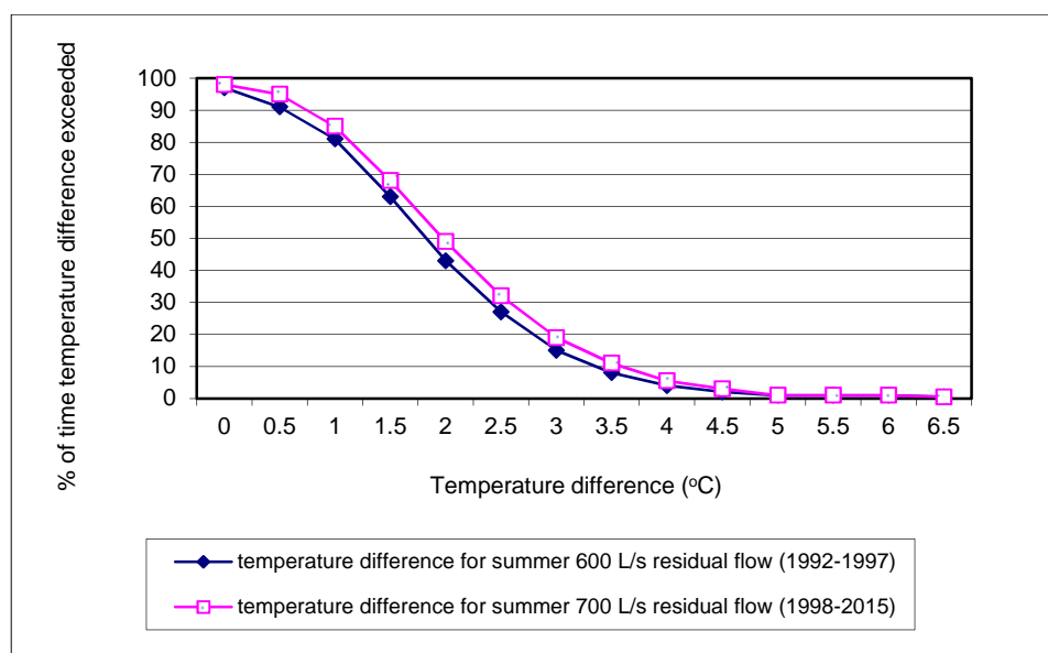
Figure 13 Exceedance time (%) for the temperature difference between natural flow upstream of weir (SH3) and residual flow downstream at Hydro Road prior to and after the summer residual flow was increased by 100 L/s
