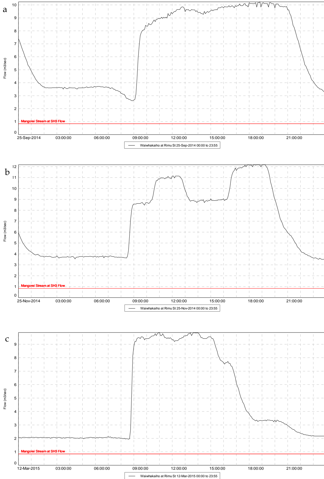
Figure 6 Examples of river flows at Rimu Street during period of 400 L/s (a), 600 L/s (b) and 700 L/s (c) residual flow releases and daylight (950 L/s) generation flow compliance during the 2014-2015 period
