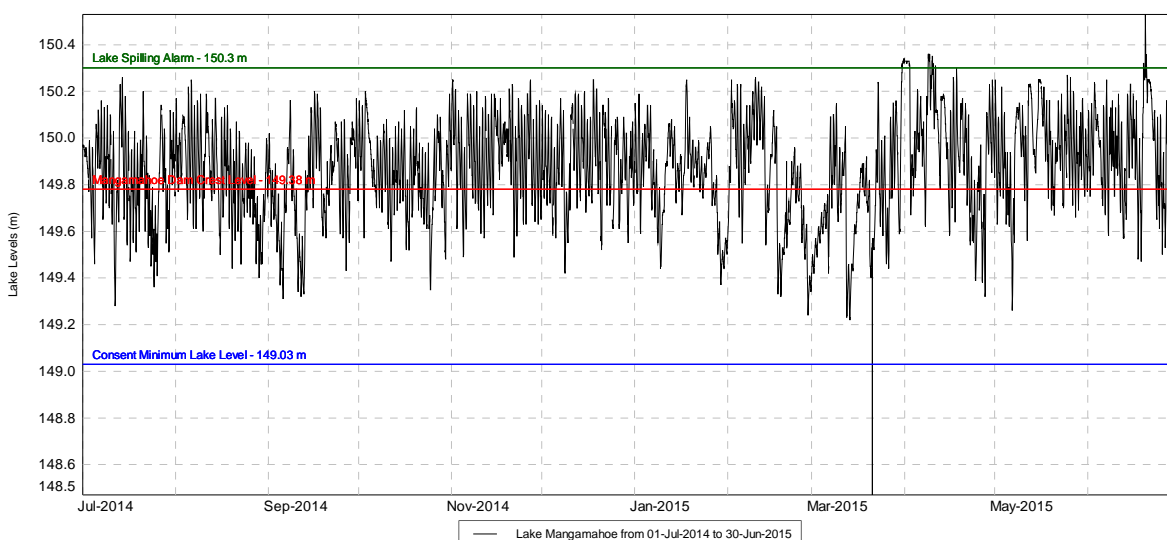
Figure 2 Lake levels (m) at Lake Mangamahoe, 1 July 2014 to 30 June 2015
