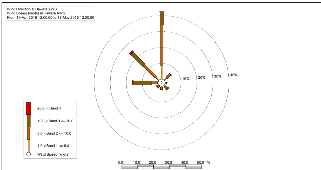
Figure 9 Wind-rose for Hawera weather station during deployment of deposition gauges, 19 April to 18 May 2016
