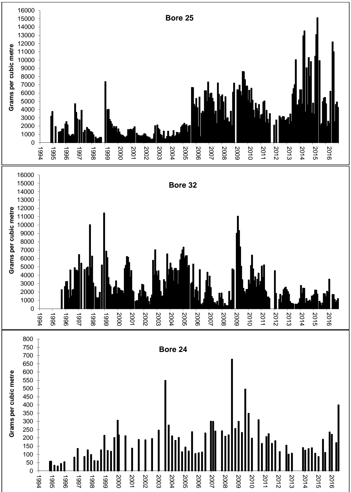
Figure 7 Total nitrogen concentration in groundwater in the vicinity of urea processing (bores 25 and 32) and the bulk storage (bore 24) areas
