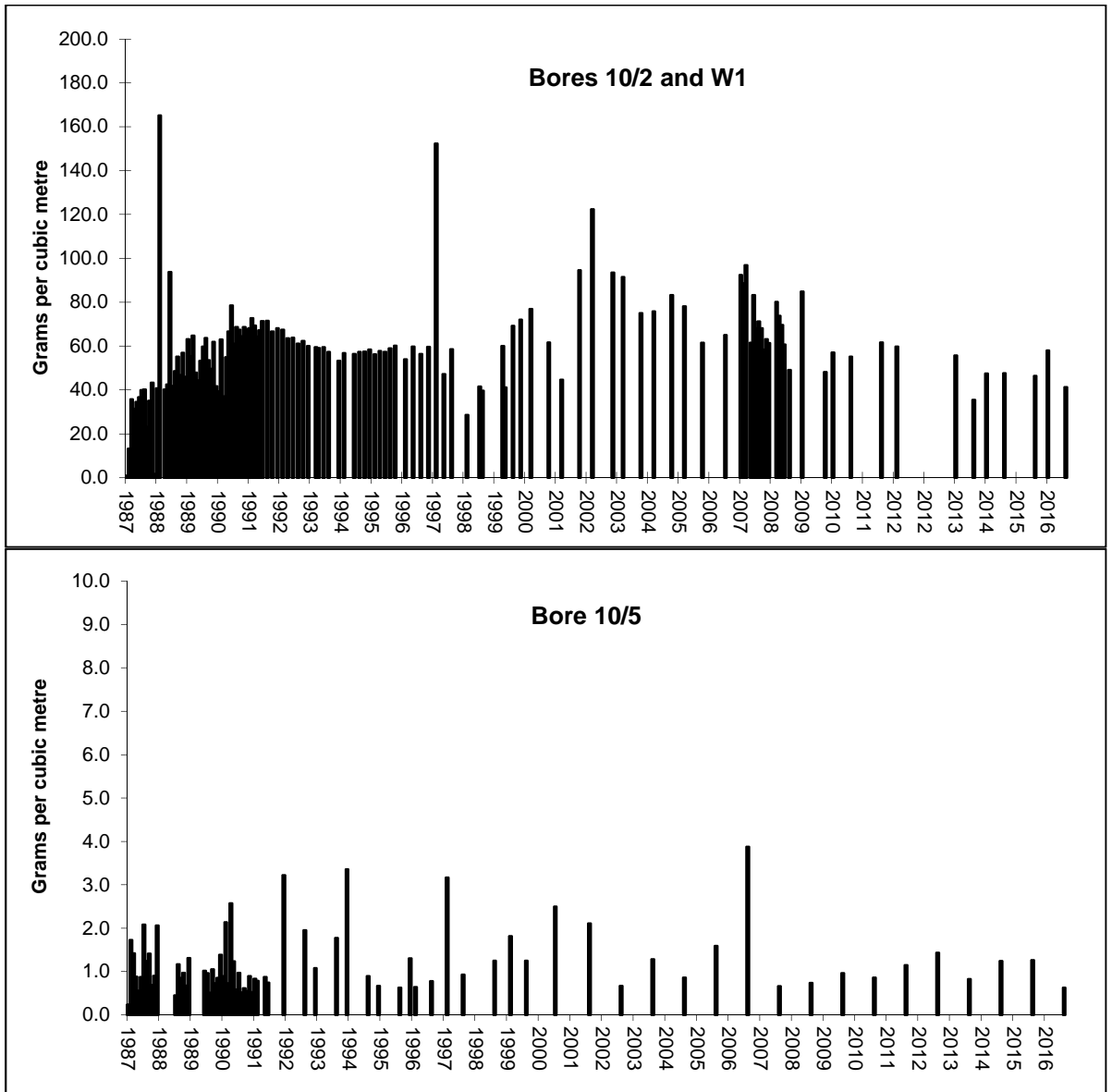
Figure 5 Total nitrogen concentrations in groundwater beneath spray irrigation areas (bores 10-2 and W1, and bore 10/5)
