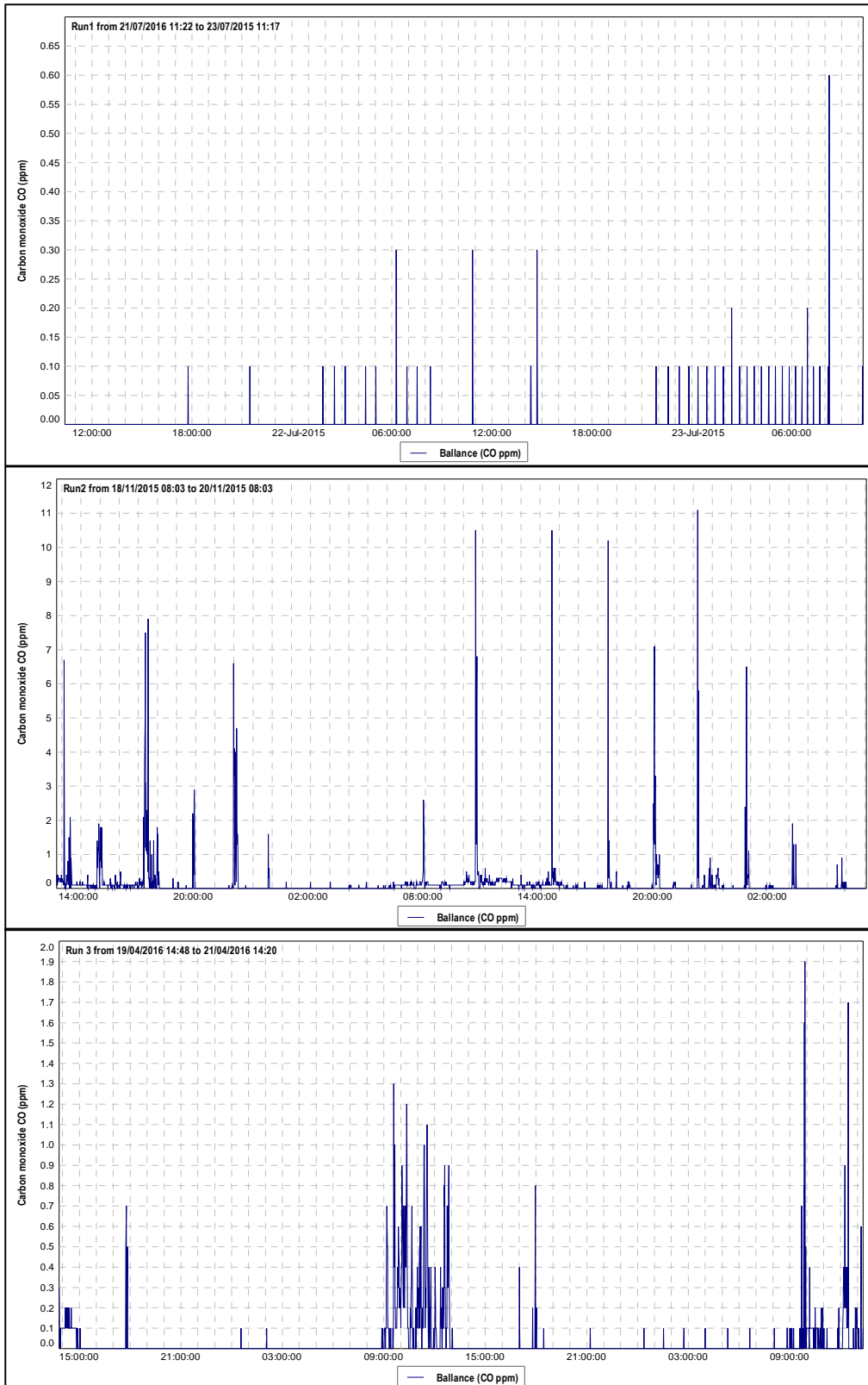
Figure 12 Graphs of ambient carbon monoxide levels in the vicinity of the ammonia urea plant, 2015-16
