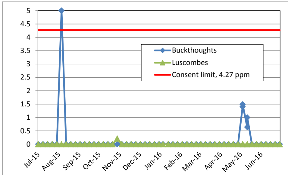
Figure 13 Atmospheric ammonia concentration at ground level on site boundary, ppm (v/v)
