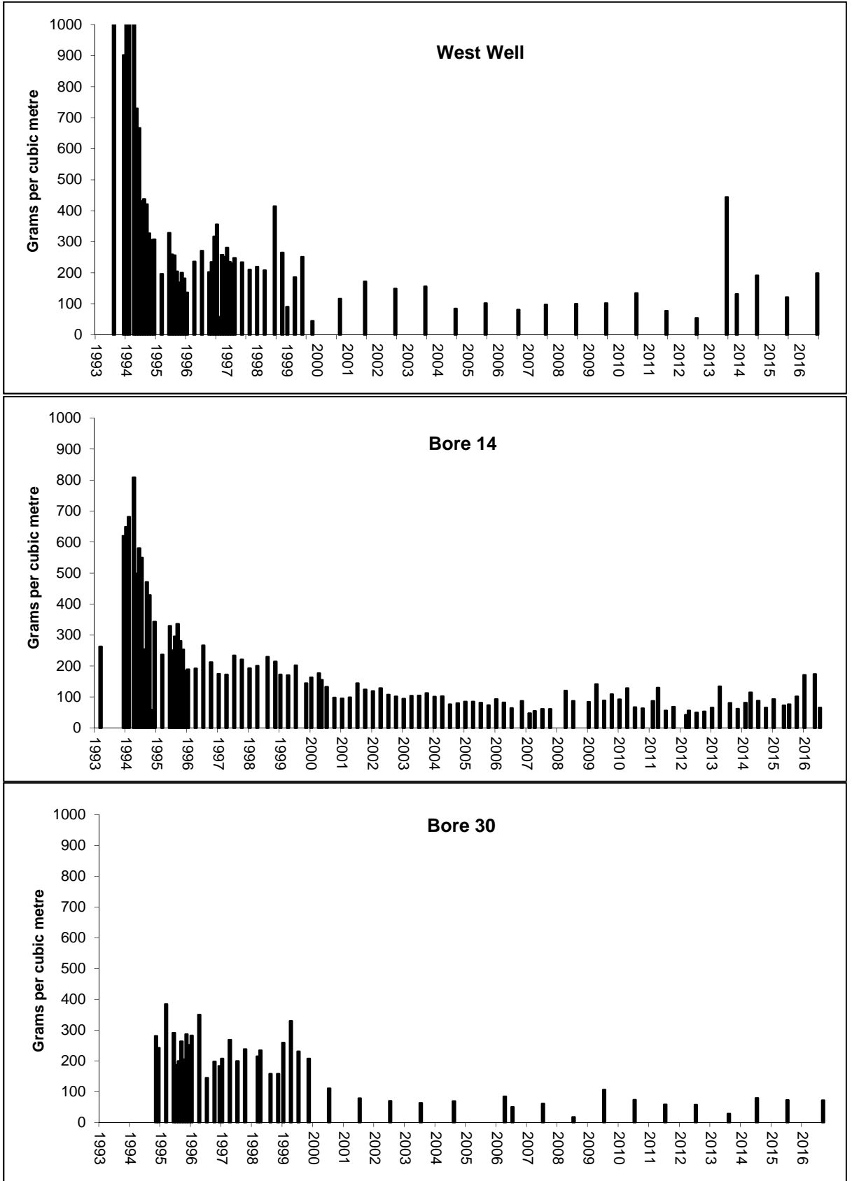
Figure 6 Total nitrogen concentration in groundwater associated with the FECB plume monitoring
