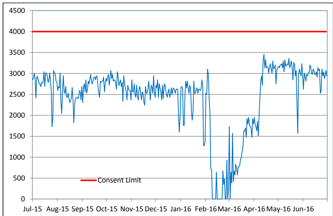
Figure 1 Daily water abstraction by Ballance Agri-Nutrients, July 2015 – June 2016, m 3
