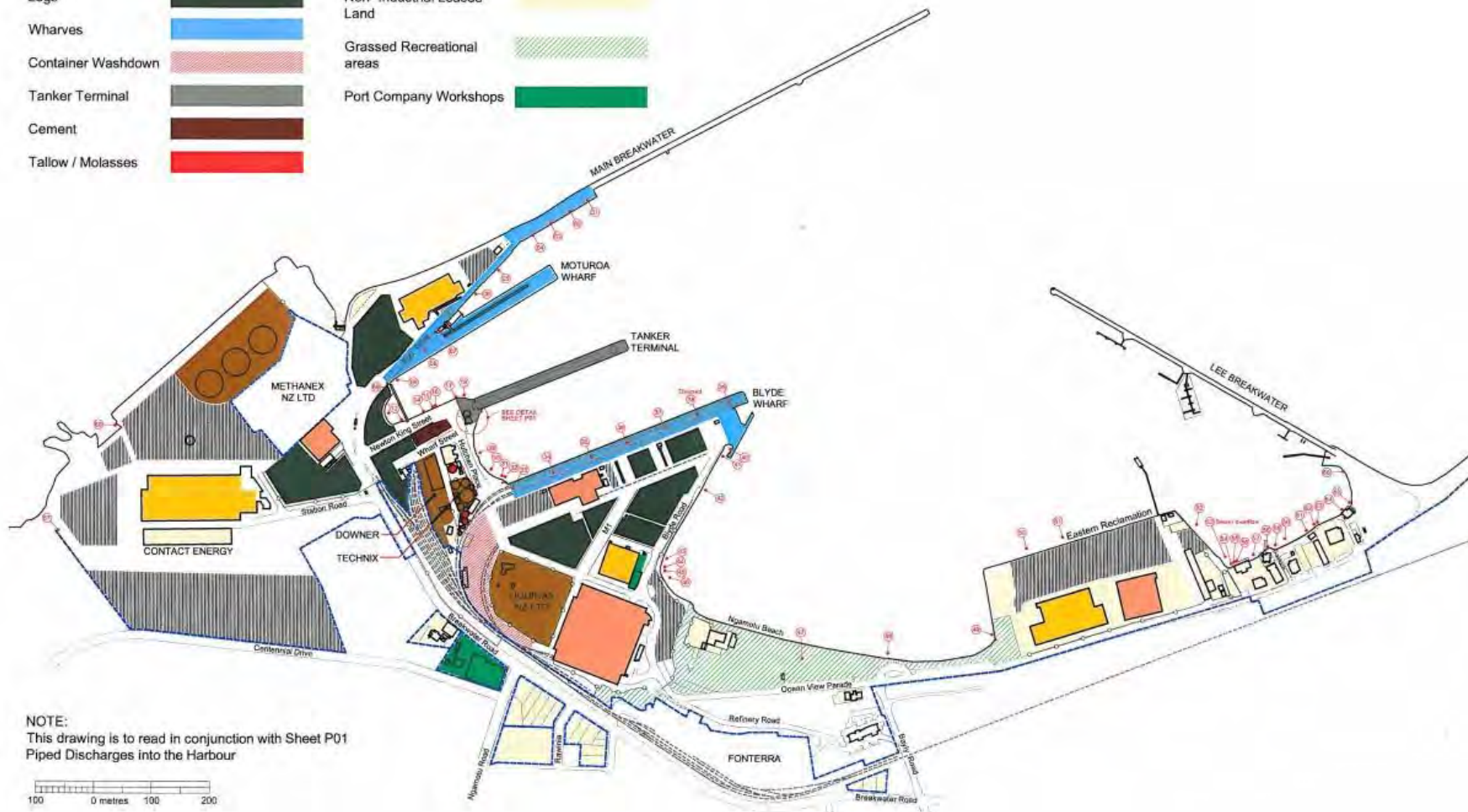
Figure 1 Land use plan of Port Taranaki showing the location of the piped stormwater discharges and the log yards
