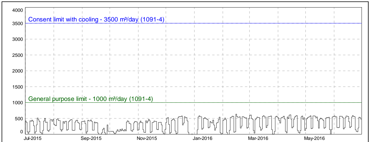
Figure 2 Daily water abstraction by Silver Fern Farms, July 2015 – June 2016, m 3
