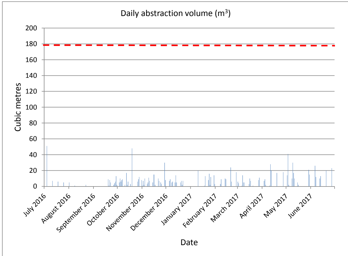
Figure 5 Daily abstraction volume for the 2016-17 period, from the Kahouri Stream (Compliance limit)
