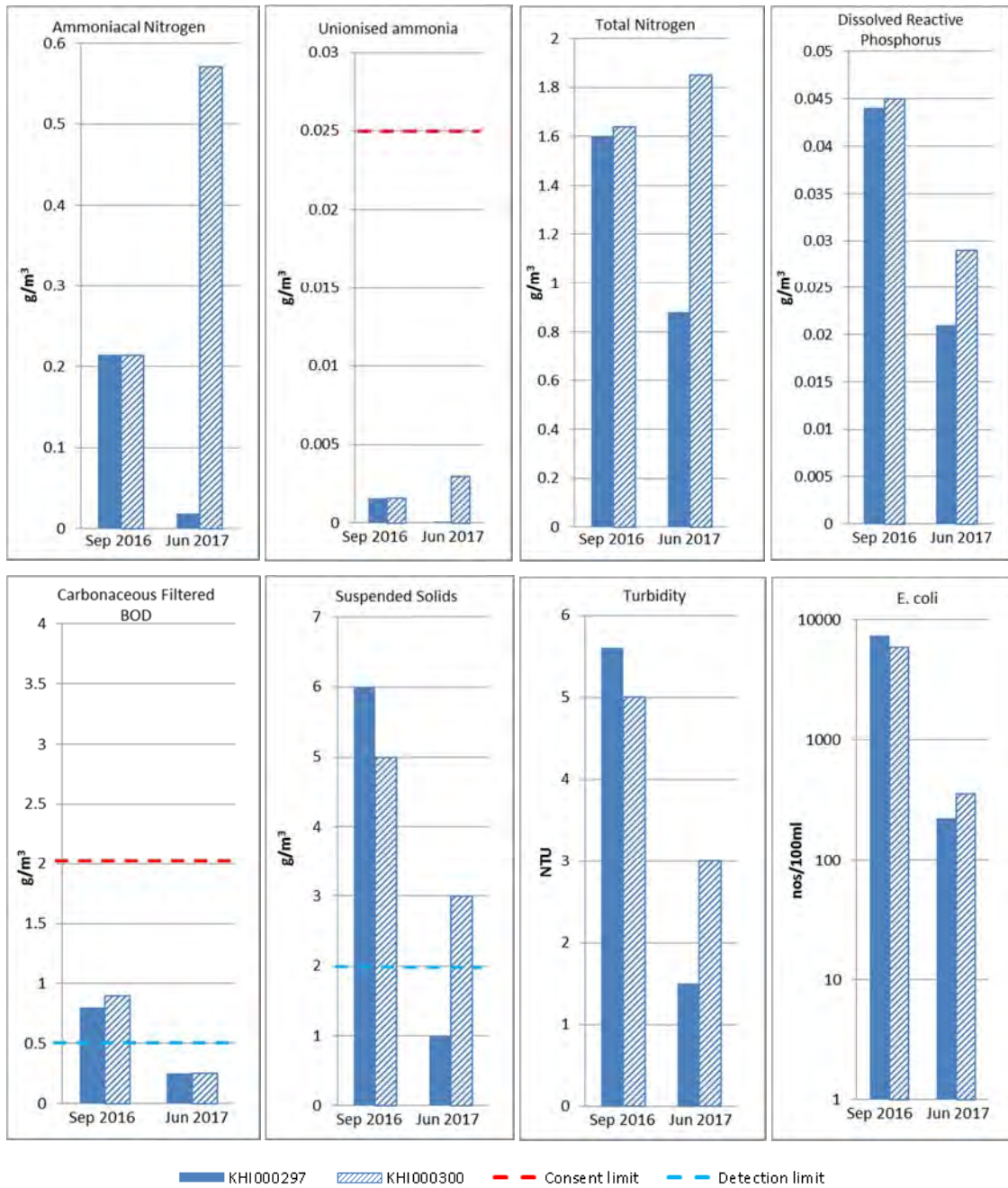
Figure 11 Sample results from the Kahouri Stream upstream and downstream of the site's wastewater discharge.
