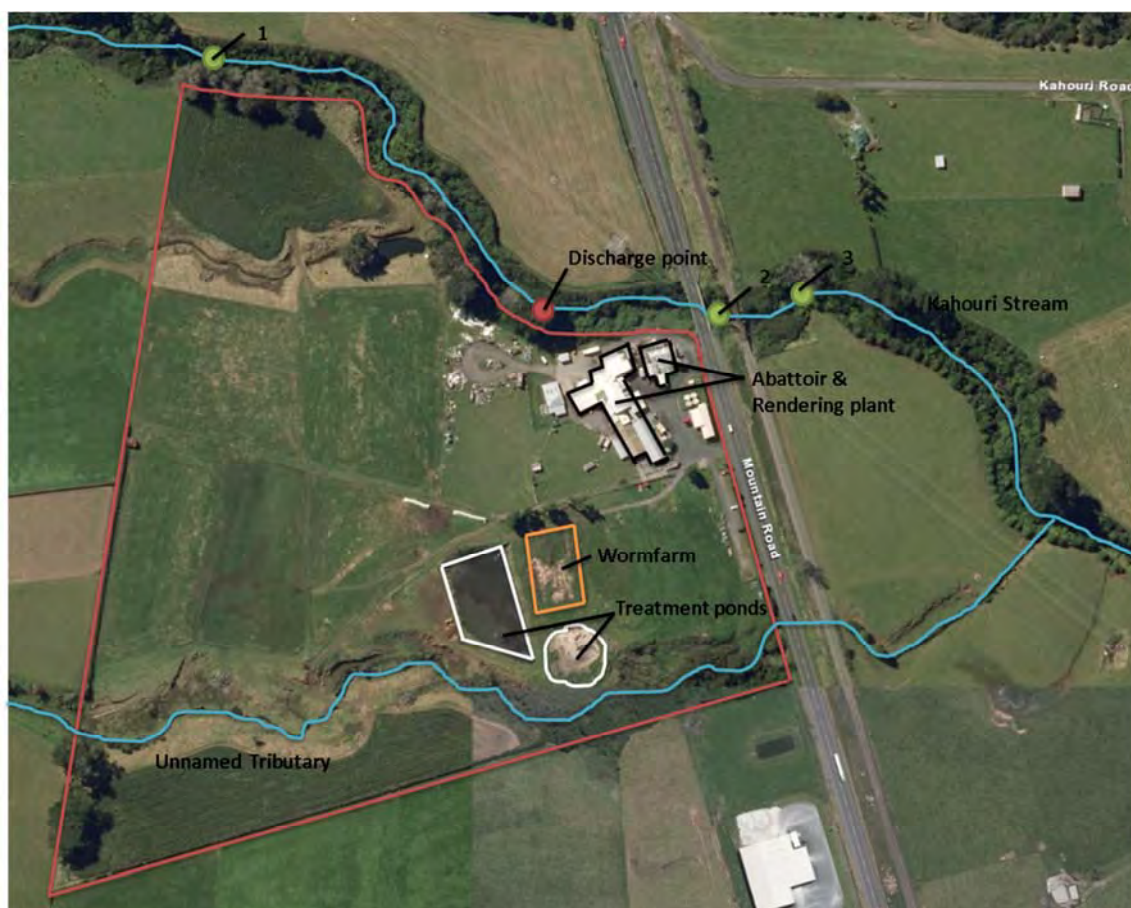
Figure 1 Ample Group Ltd meat processors site layout and biomonitoring sites, in relation to the discharge point
