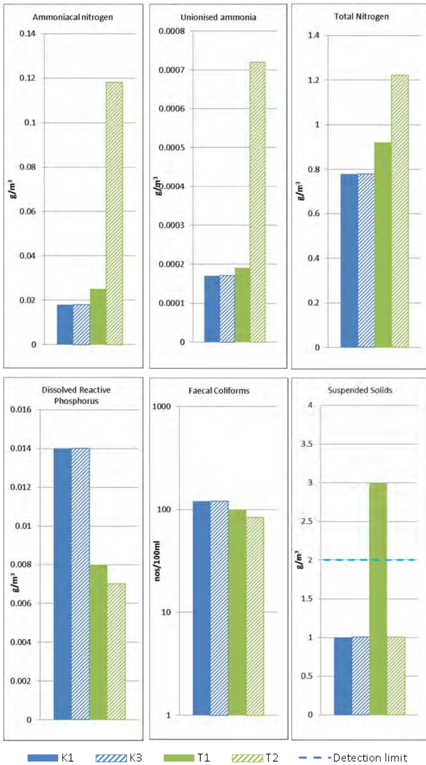
Figure 12 Water quality sampling results for the first synoptic survey
