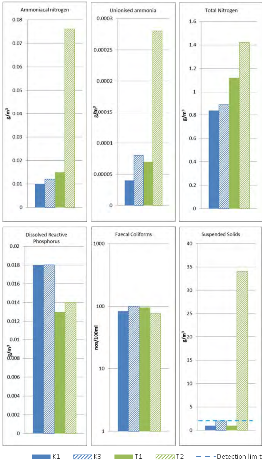
Figure 13 Water quality sampling results for the second synoptic survey
