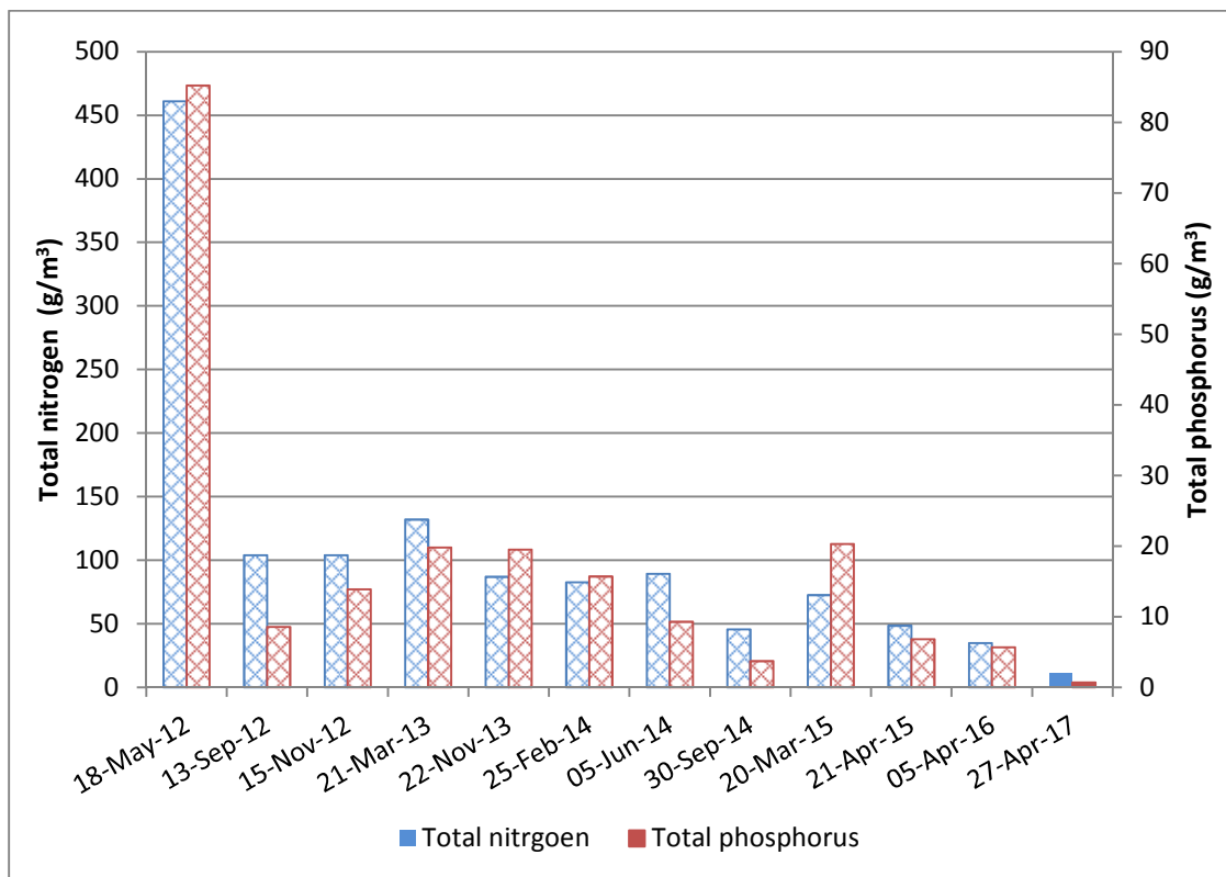
Figure 4 Concentrations of total nitrogen and total phosphorus in the irrigated wastewater. The solid bars indicate the sample collected in the 2016-2017 monitoring period
