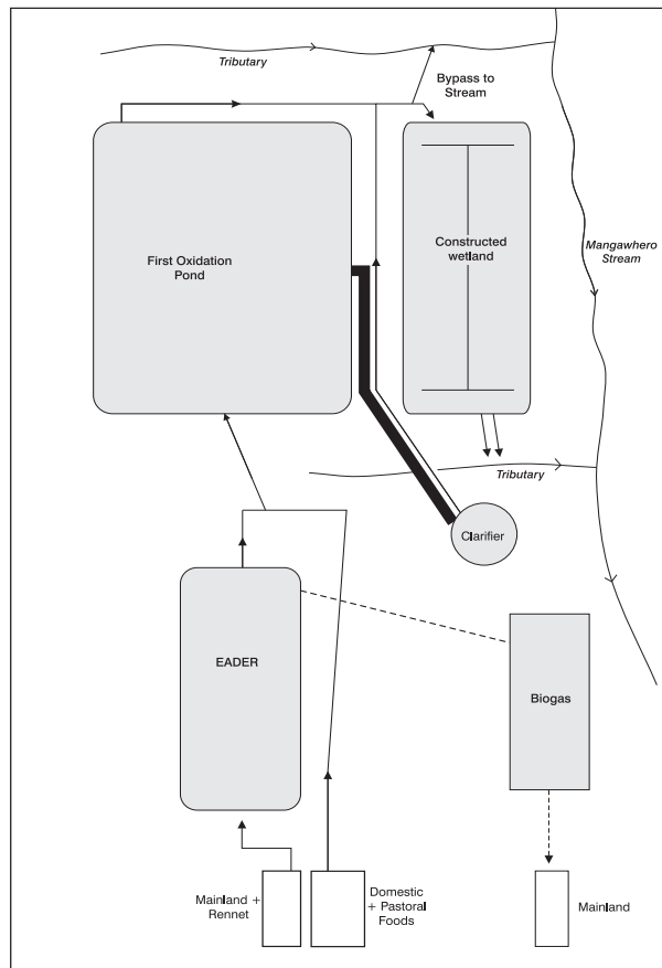
Figure 1 Schematic layout of Eltham wastewater treatment plant as operational prior to the 2010-2011 period
