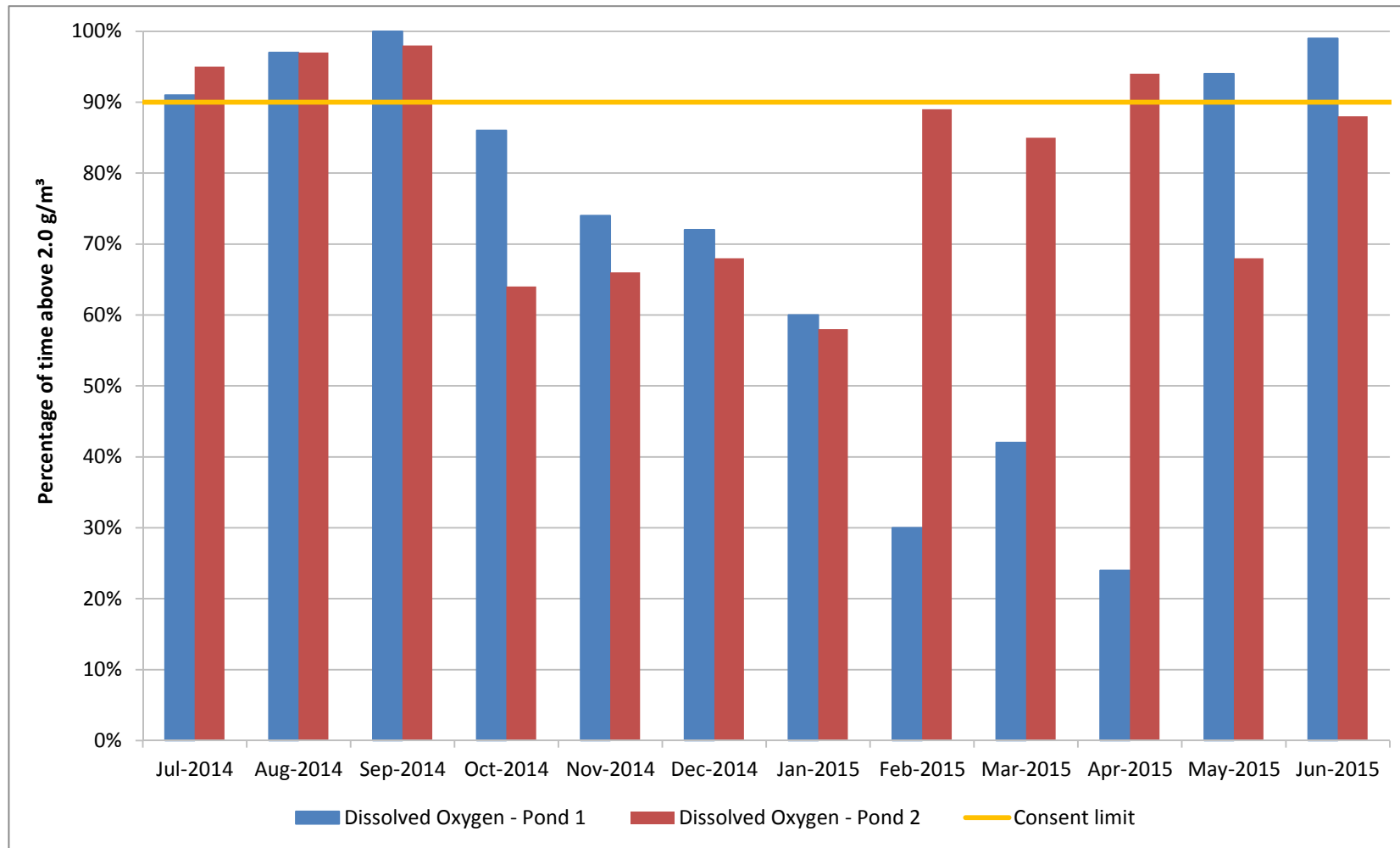
Figure 2 Compliance of DO concentration ( \text{g/m}^3 ) with consent conditions in the primary and secondary oxidation ponds 2014-2015 (between hours of 1100 – 1400). Data from pond outlet.
