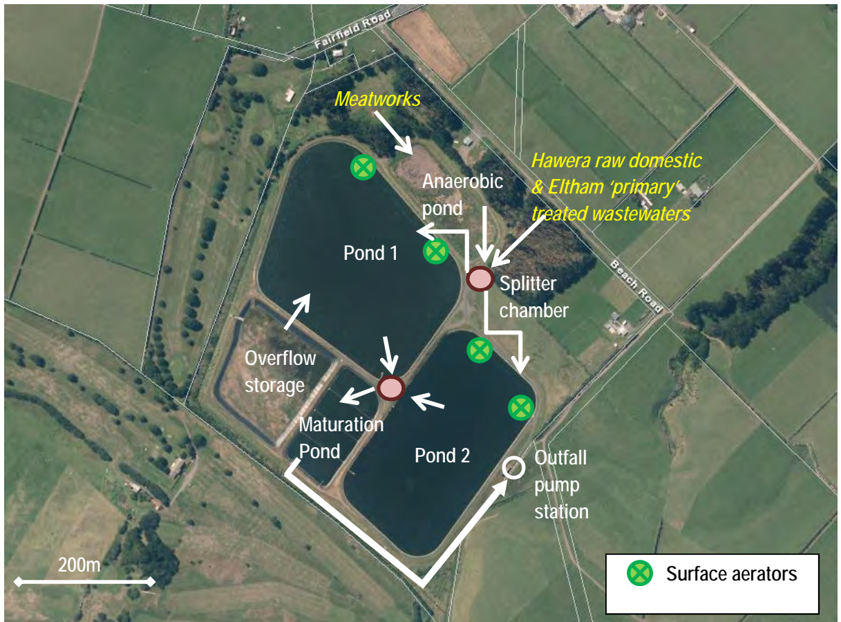
Figure 1 Configuration of the HWWTP (adapted from NIWA 2012)
