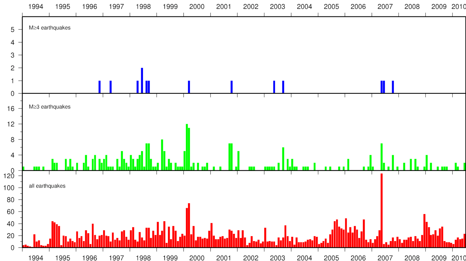
Figure 7. A histogram of the number of earthquakes less than 50 km deep that have occurred each month between January 1994 and June 2010 in the area shown in Figure 1. Three separate histograms are shown: all earthquakes (bottom), those of magnitude 3 and above (centre) and those of magnitude 4 and above (top).
