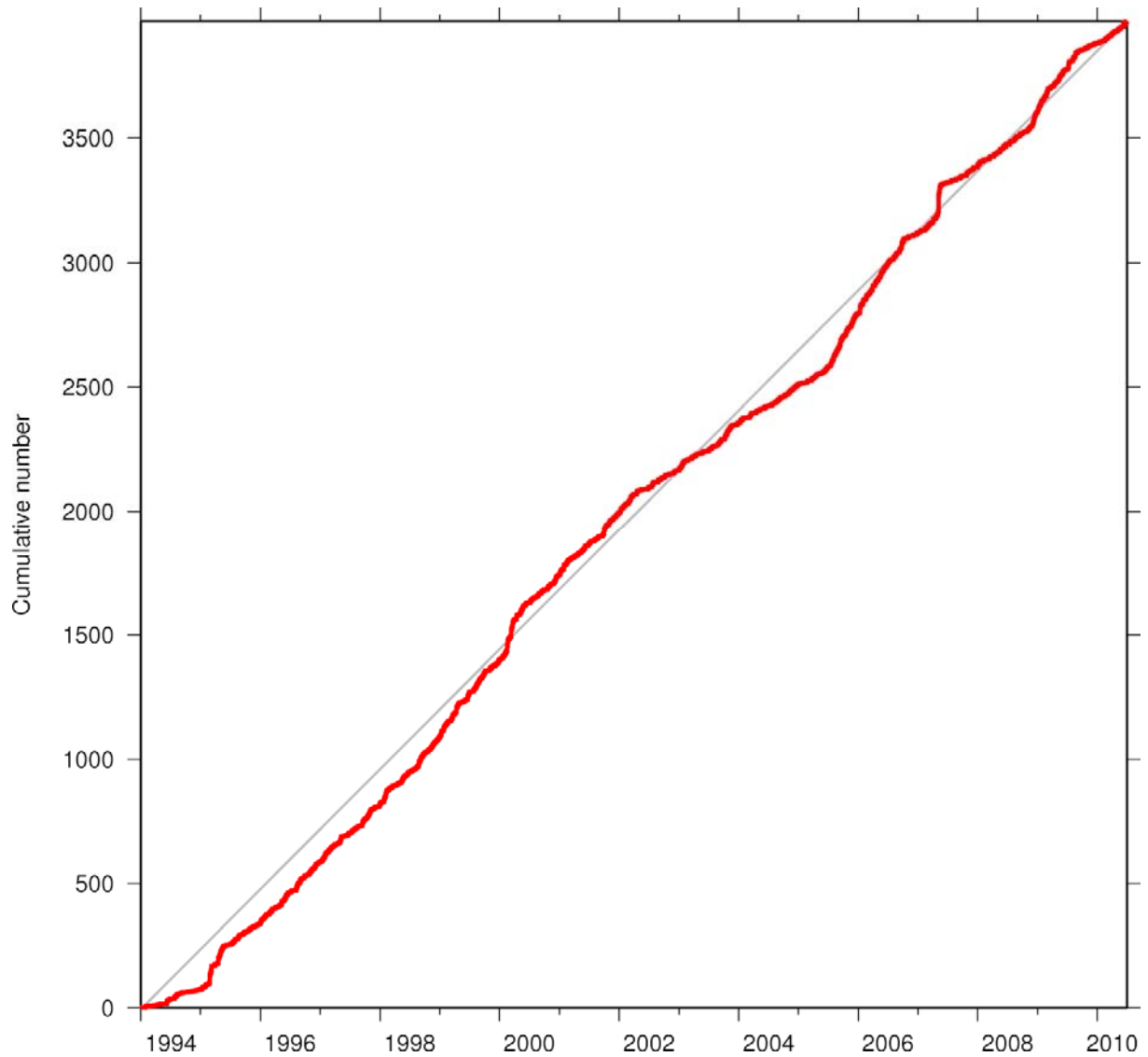
Figure 8. The cumulative number of earthquakes (red line) less than 50 km deep located in the area shown in Figure 1 between January 1994 and June 2010. The grey line shows the mean rate.
