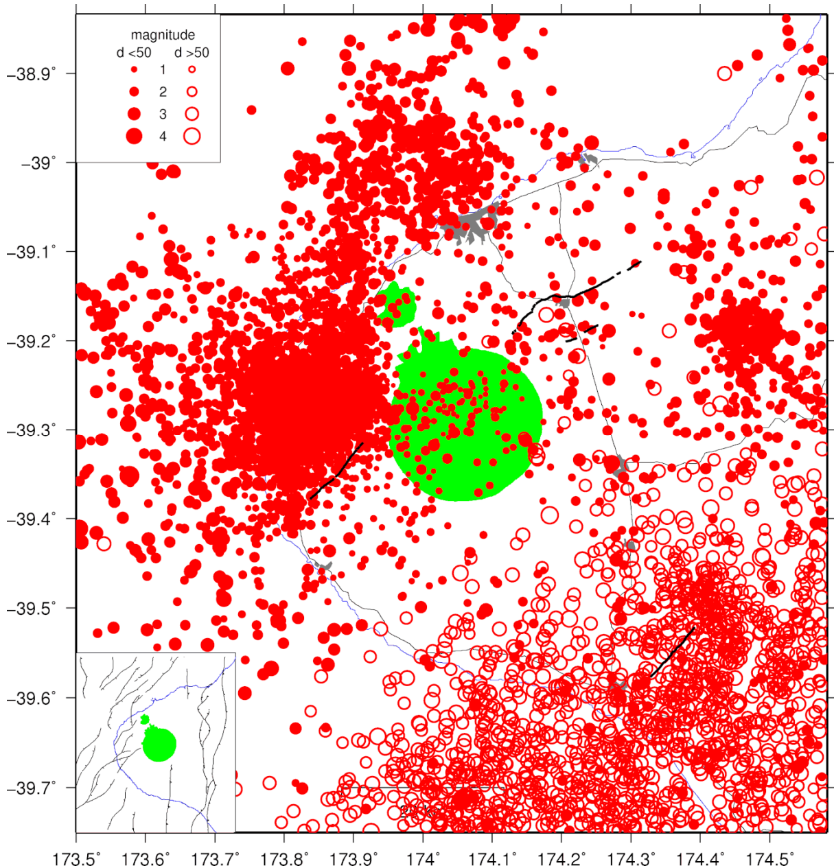
Figure 5. A map of earthquakes located in Taranaki between January 1994 and June 2010. Data are from the GNS earthquake database. Closed circles indicate earthquakes less than 50 km deep and open circles those more than 50 km deep. The size of the symbol is proportional to the magnitude of the earthquake, and representative symbols are shown in the top left corner of the diagram. Population centres are shaded dark grey and Egmont National Park is shaded green. Major roads and mapped faults (thick black lines) are also shown. The lower left inset shows faults that offset the basement rocks but are not considered active faults.
