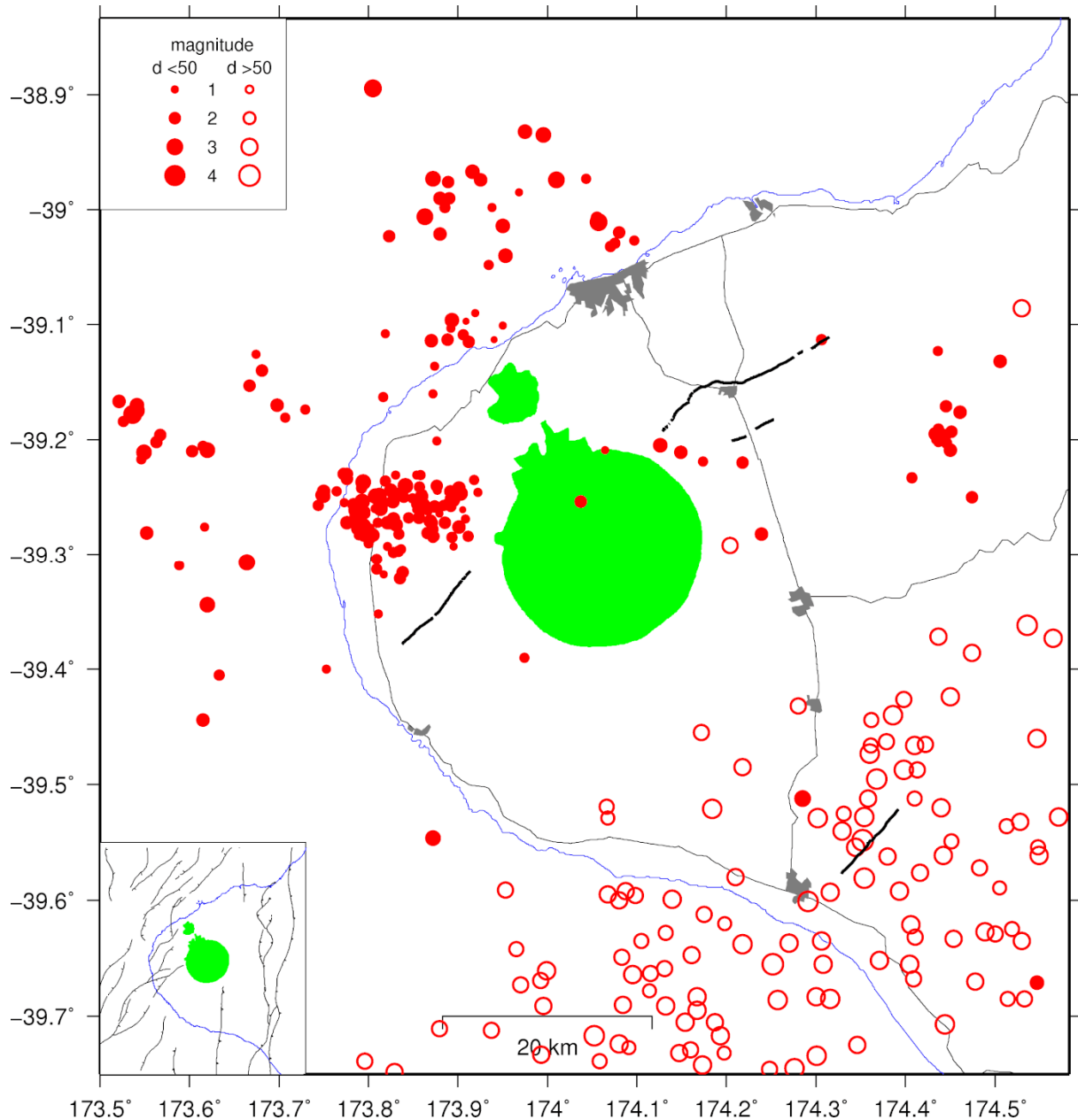
Figure 2. A map of all earthquakes located in Taranaki between July 2009 and June 2010. Closed circles indicate earthquakes less than 50 km deep and open circles those more than 50 km deep. The size of the symbol is proportional to magnitude of the earthquake, and representative symbols are shown in the top left corner of the diagram. Population centres are shaded dark grey and Egmont National Park is shaded green. Major roads and mapped active faults (thick black lines) are also shown. The lower left inset shows faults that offset the basement rocks but are not considered active faults.
