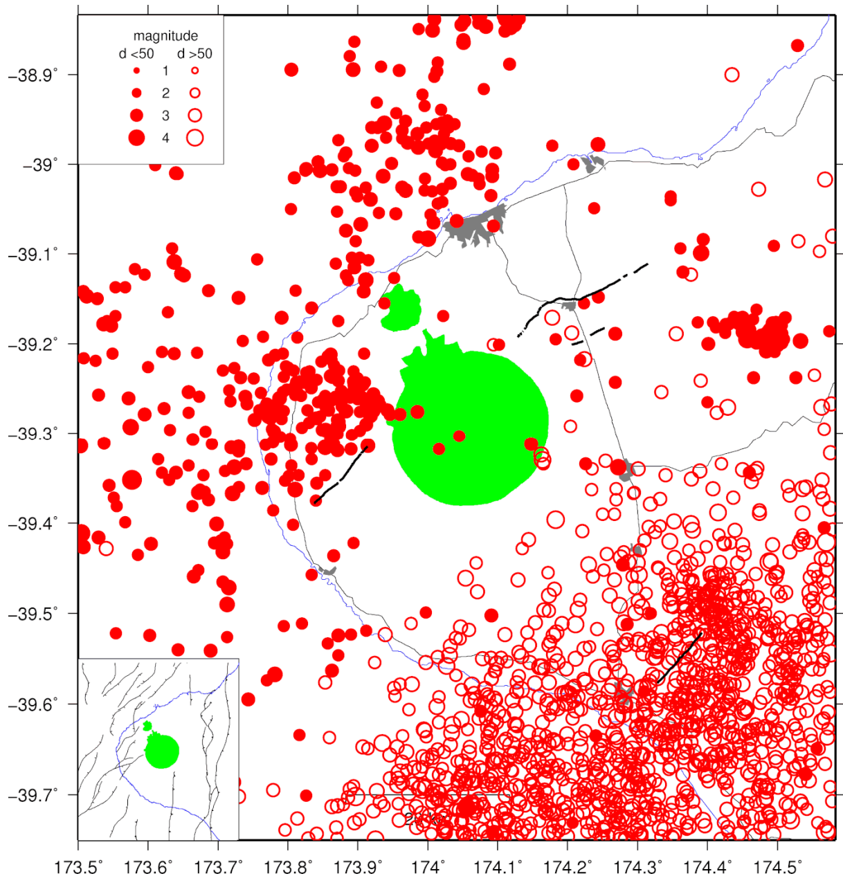
Figure 6. A map of earthquakes of M2.7 and larger located in Taranaki between January 1994 and June 2010. Data are from the GNS earthquake database. Closed circles indicate earthquakes less than 50 km deep and open circles those more than 50 km deep. The size of the symbol is proportional to the magnitude of the earthquake, and representative symbols are shown in the top left corner of the diagram. Population centres are shaded dark grey and Egmont National Park is shaded green. Major roads and mapped faults (thick black lines) are also shown.
