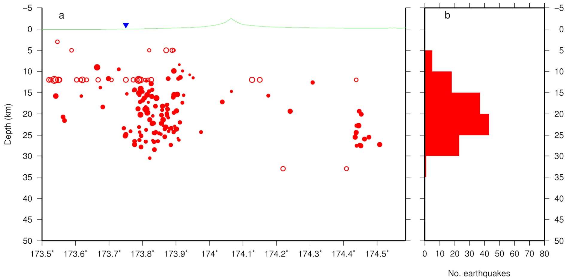
Figure 4a. An east-west cross-section showing earthquakes less than 50 km deep located in Taranaki between July 2009 and June 2010. The symbols are the same as Figure 3, closed circles for earthquakes for which the depth was calculated and open circles for those for which the depth was fixed. Topography is shown in the upper part of the diagram, with the inverted triangle marking the position of the coast at Cape Egmont. The horizontal: vertical scale is 1:1. The location of the cross-section is shown as a dashed box in Figure 3.
