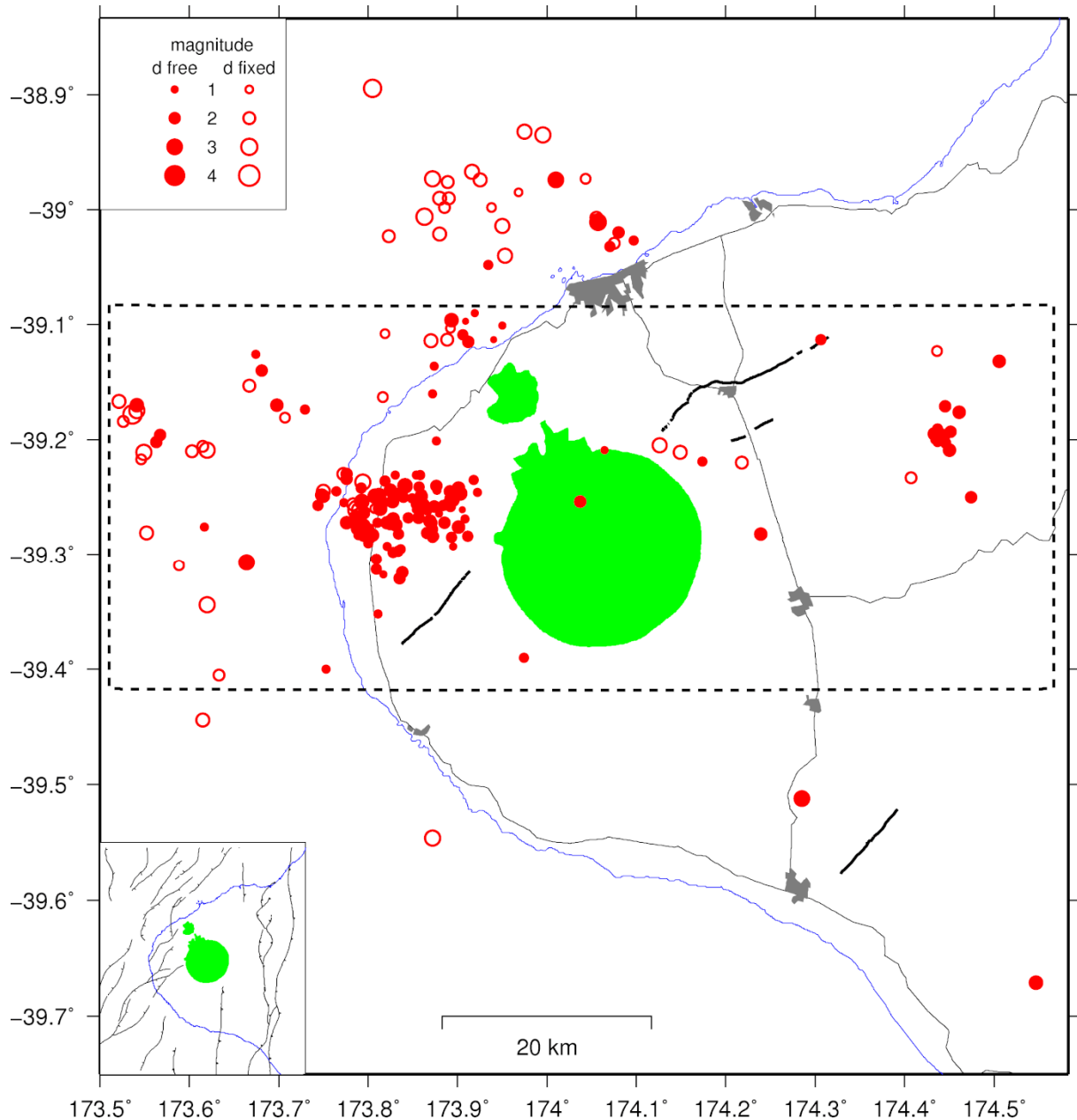
Figure 3. A map of earthquakes less than 50 km deep located in Taranaki between July 2009 and June 2010. Closed circles indicate earthquakes for which a depth was calculated and open circles those for which a depth could not be calculated and was therefore fixed at some appropriate value. The size of the symbol is proportional to the magnitude of the earthquake, and representative symbols are shown in the top left corner of the diagram. Population centres are shaded dark grey and Egmont National Park is shaded green. Major roads and mapped active faults (thick black lines) are also shown. The lower left inset shows faults that offset the basement rocks but are not considered active faults. The dashed box marks the location of the cross-section in Figure 4a.
