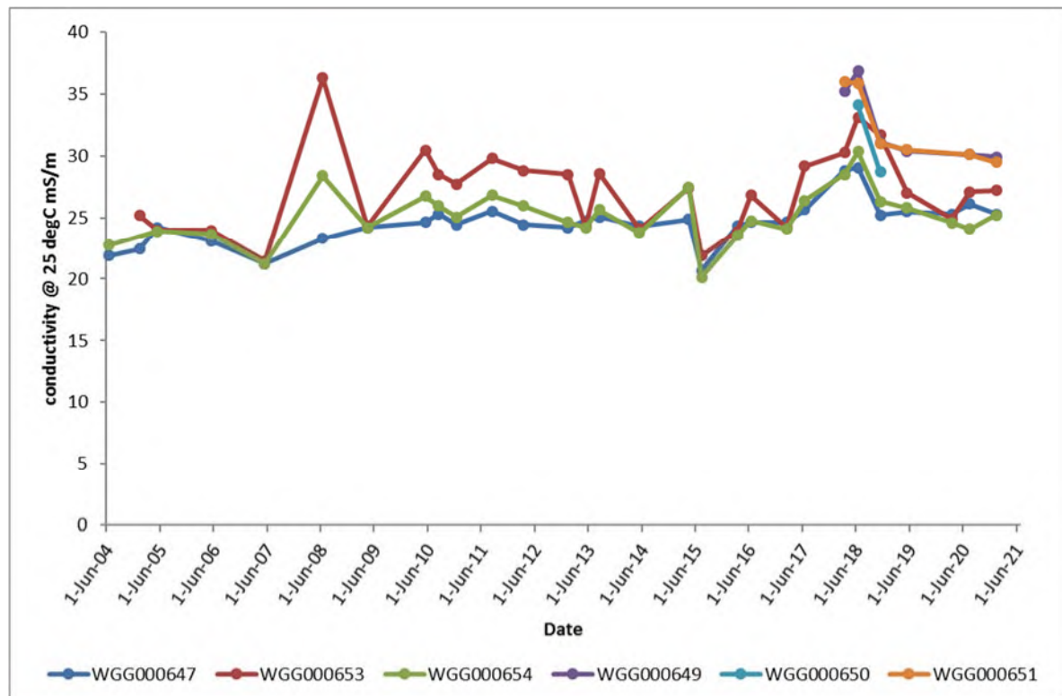
Figure 7 Conductivity levels found in surface water at the Central landfill site, 2004-2021
