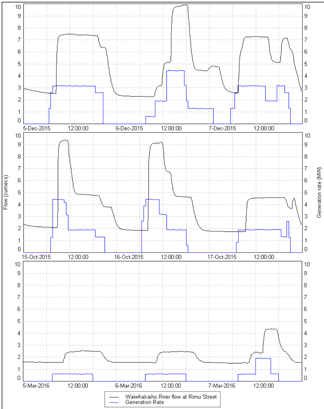
Figure 6 Flow variation in the Waiwhakaiho River at Rimu Street as a result of generation at the Mangorei Power Station.
