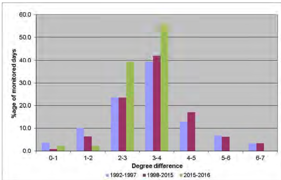
Figure 12 The distribution of maximum daily temperature differences (Hydro Road minus Egmont Village), displayed as a percentage of total days monitored. Data has been split into 600 L/s residual flow (1992-1997) and 700 L/s residual flow (1998 – present), and is for January to March only.
