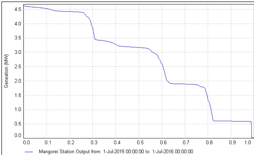
Figure 5 Exceedance time (%) for generation at the Mangorei Power house, 1 July 2015 – 1 July 2016, 9am to 5pm only.
