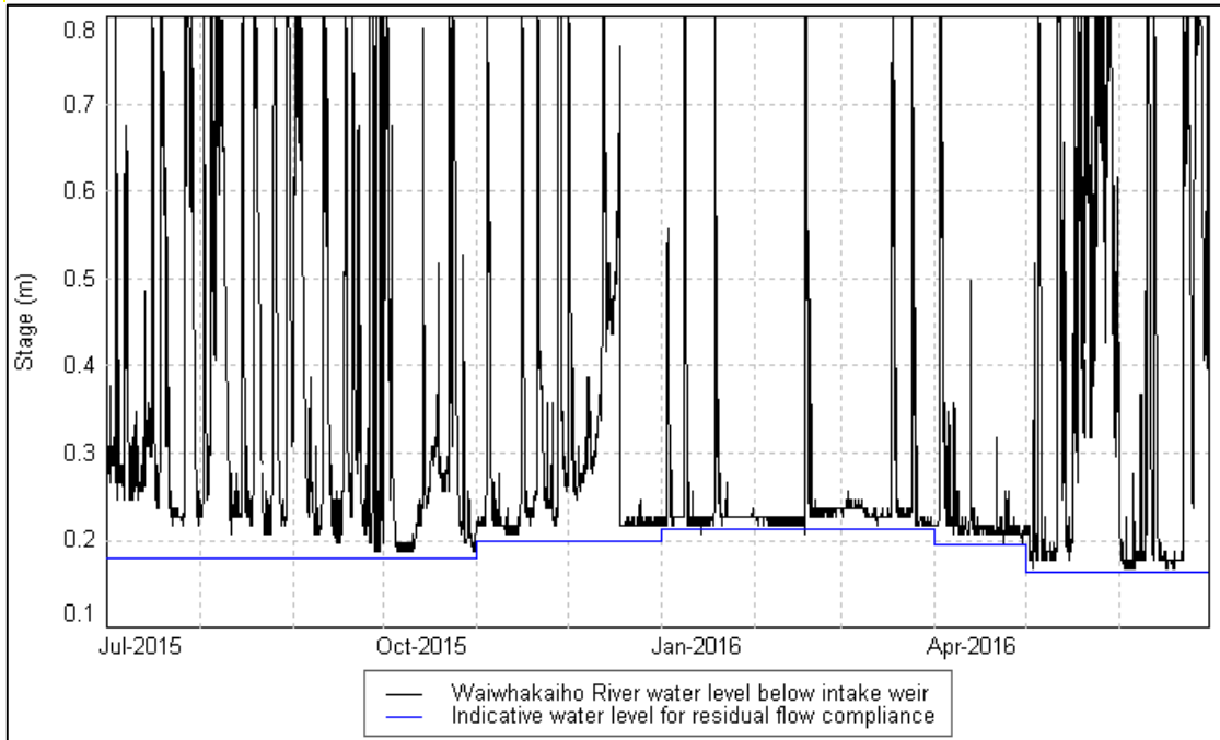
Figure 3 Water level downstream of the intake weir, compared with indicative water level required to ensure residual flow compliance.
