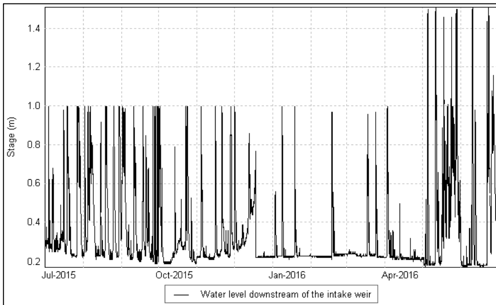
Figure 2 Water level data recorded by Trustpower, downstream of the intake weir.
