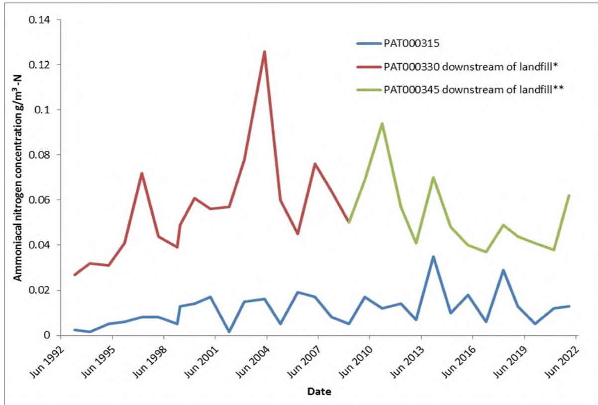
Figure 7 Graph showing ammoniacal nitrogen levels in the Patea Stream up and downstream of the landfill (where comparative data is available)
