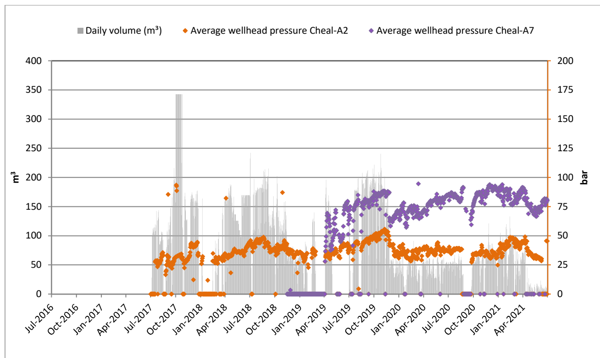
Figure 9 Cheal-A wellsite: Daily injection volumes and injection pressures (2017-2021)
