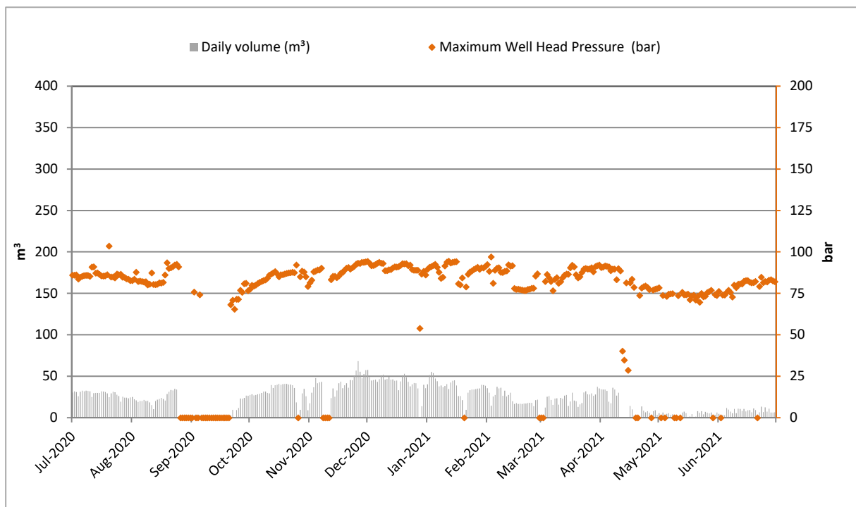
Figure 8 Cheal-A7 well: Daily injection volumes and injection pressures (2020-2021)
