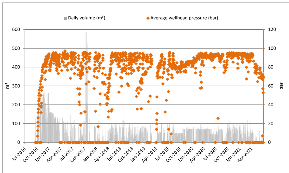
Figure 11 Cheal-B3 well: Daily injection volumes and injection pressures (2016-2021)
