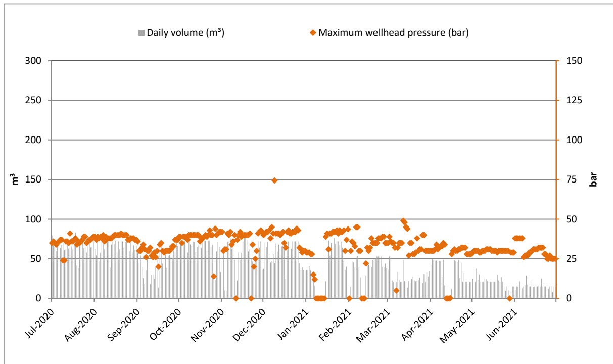
Figure 12 Cheal-E4 well: Daily injection volumes and injection pressures (2020-2021)
