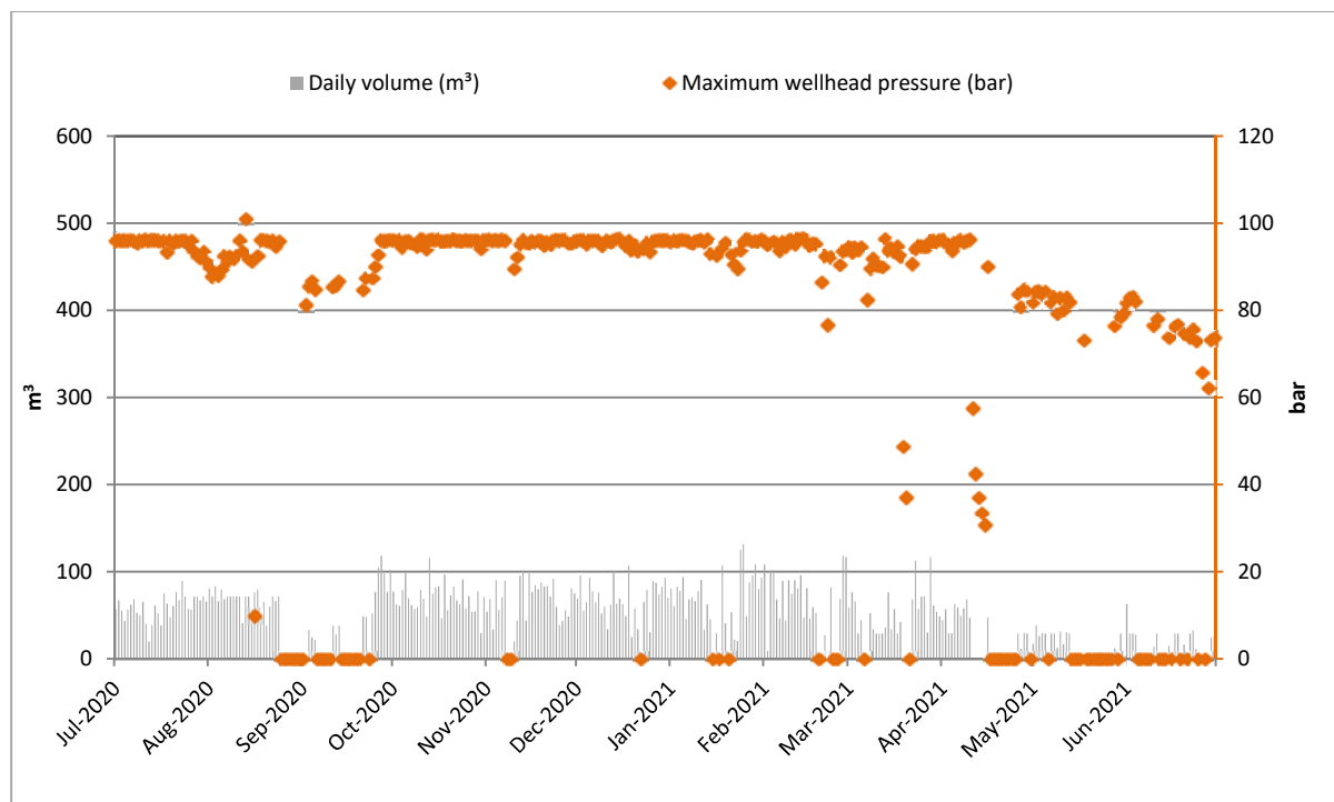
Figure 10 Cheal-B3 well: Daily injection volumes and injection pressures (2020-2021)
