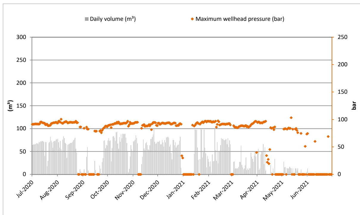
Figure 4 Cheal-A4 well: Daily injection volumes and injection pressures (2020-2021)
