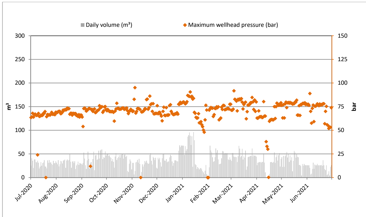
Figure 13 Cheal-E7 well: Daily injection volumes and injection pressures (2020-2021)
