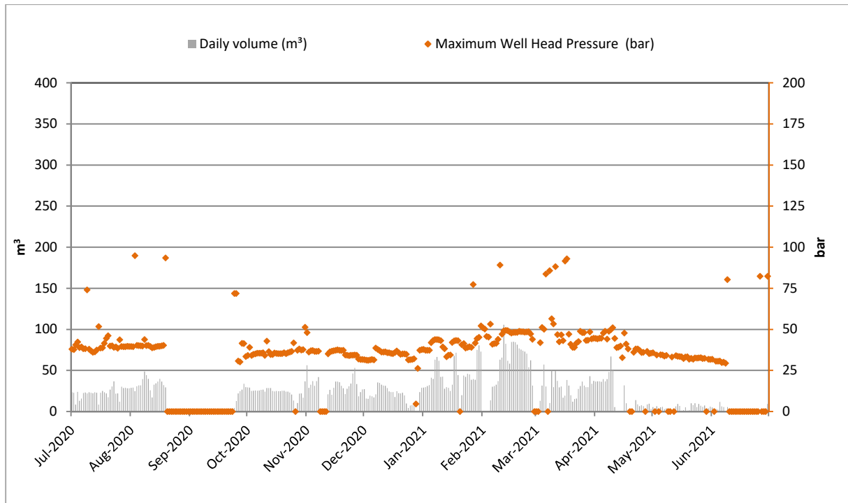
Figure 7 Cheal-A2 well: Daily injection volumes and injection pressures (2020-2021)
