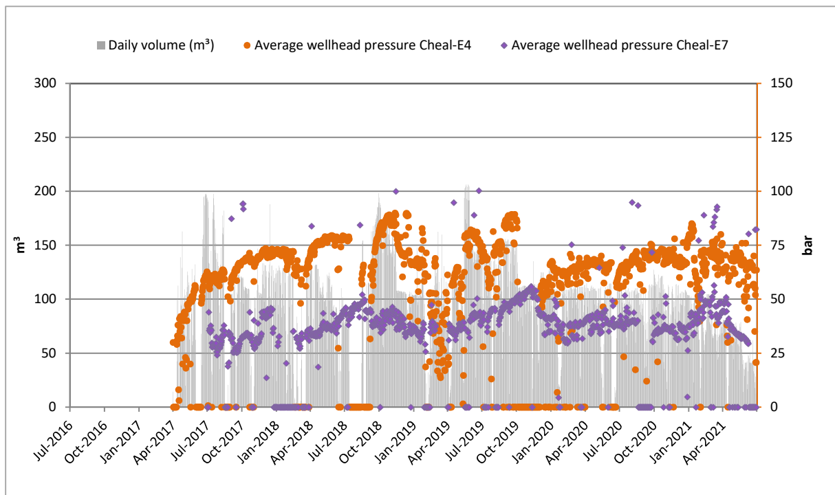
Figure 14 Cheal-E wellsite: Daily injection volumes and injection pressures (2016-2021)
