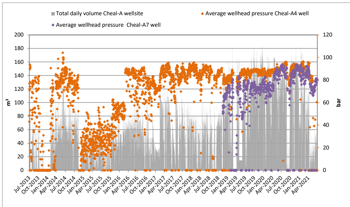
Figure 6 Cheal-A wellsite: Daily injection volumes and injection pressures (2013-2021)
