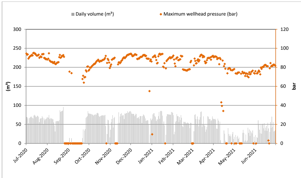
Figure 5 Cheal-A7 well: Daily injection volumes and injection pressures (2020-2021)
