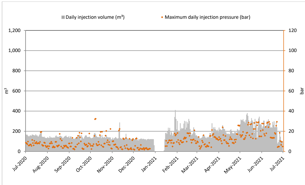
Figure 10 Tuhua-B wellsite: McKee-1 Disposal well daily injection volume and pressure (2020-2021)
