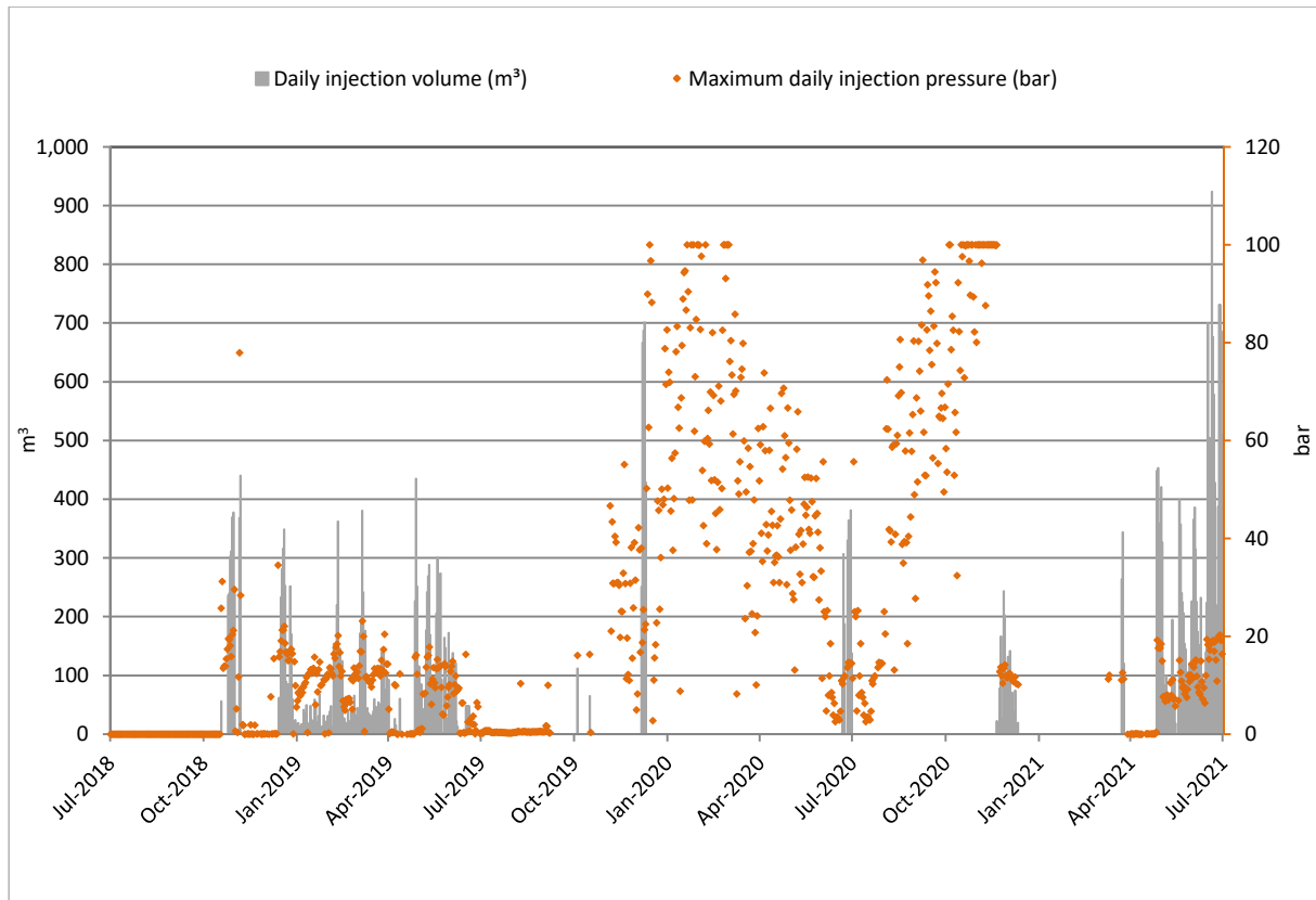
Figure 9 McKee-B wellsite: McKee-4 well daily injection volume and pressure (2018-2021)
