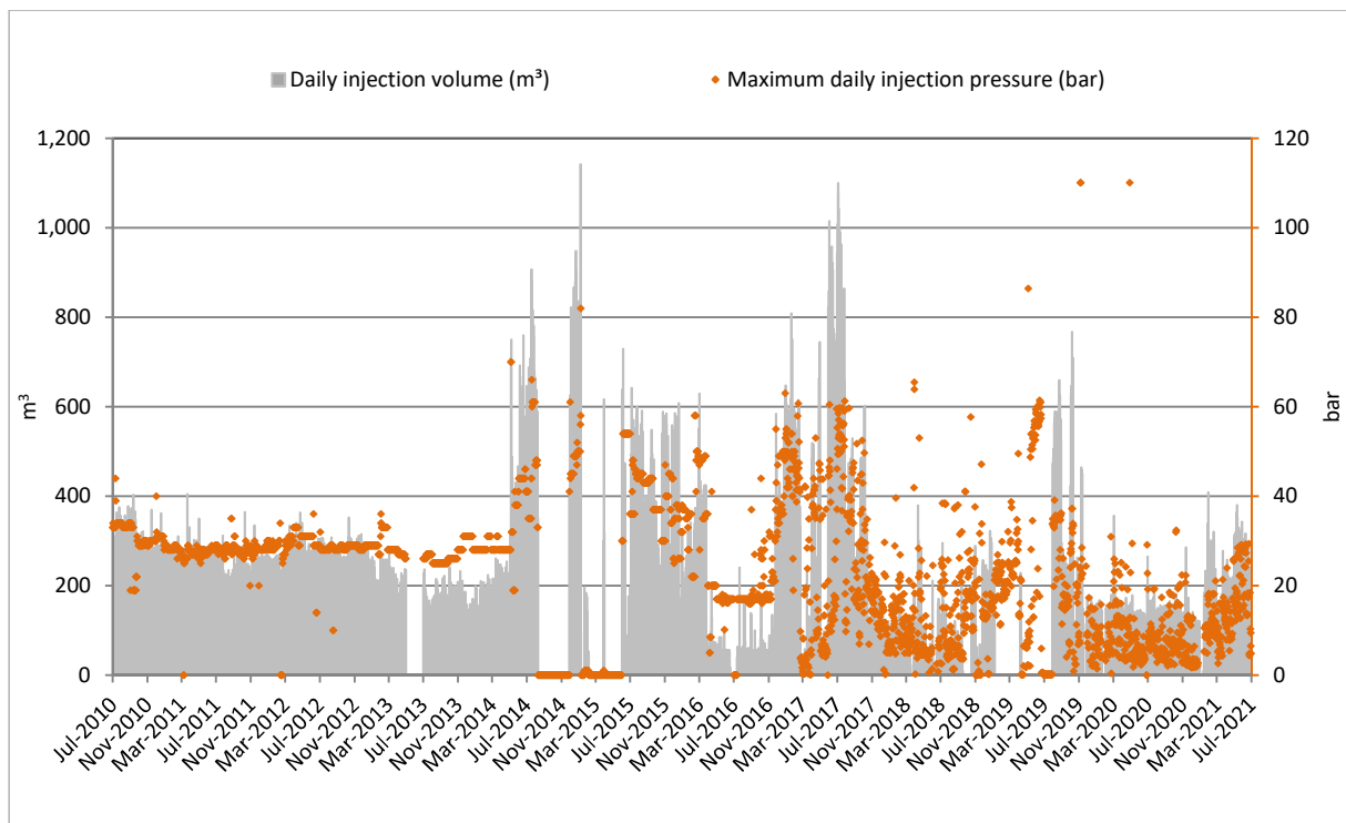
Figure 11 Tuhua-B wellsite: McKee-1 Disposal well daily injection volume and pressure (2010-2021)
