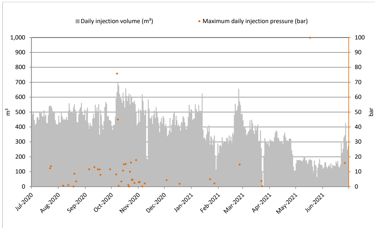
Figure 12 Tuhua-B wellsite: Tuhua-6 well daily injection volume and pressure (2020-2021)
