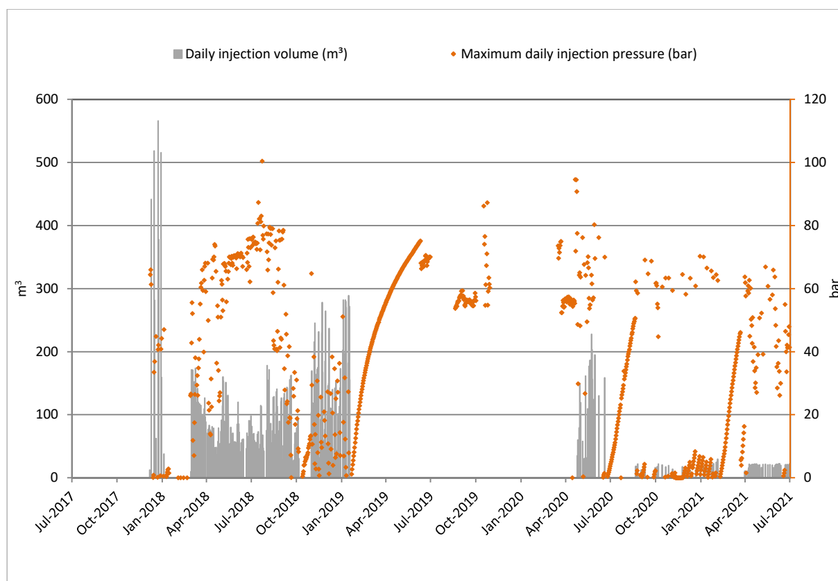
Figure 8 KA1/7/19/20 wellsite: KA1 well daily injection volume and pressure (2017-2021)
