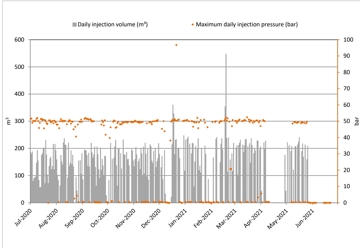
Figure 5 KA9 wellsite: KA16 well daily injection volume and pressure (2020-2021)
