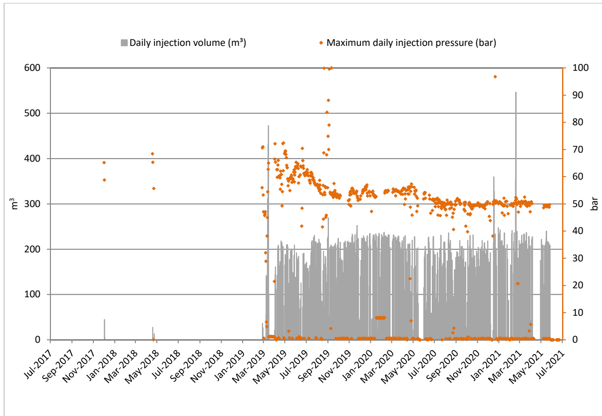
Figure 6 KA9 wellsite: KA16 well daily injection volume and pressure (2017-2021)
