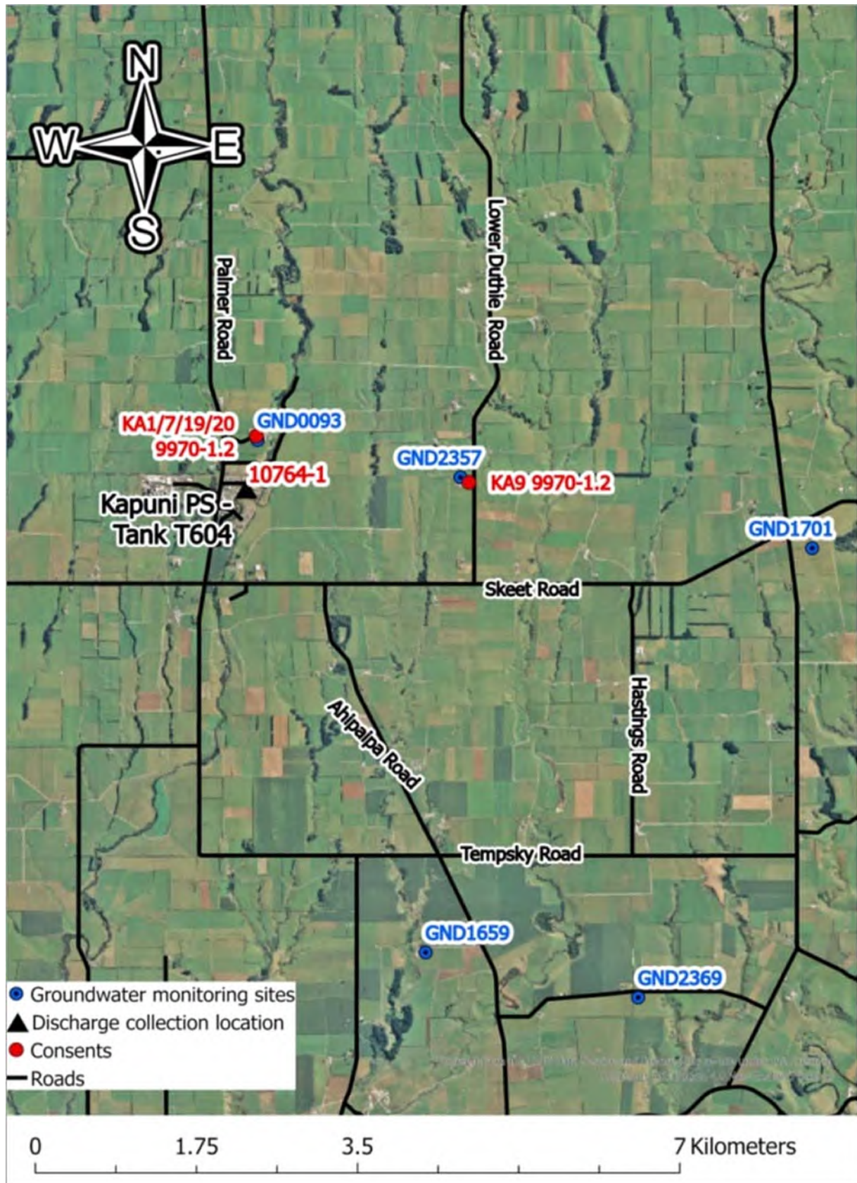
Figure 4 Locations of monitoring sites in relation to the Company's Kapuni DWI wellsites
