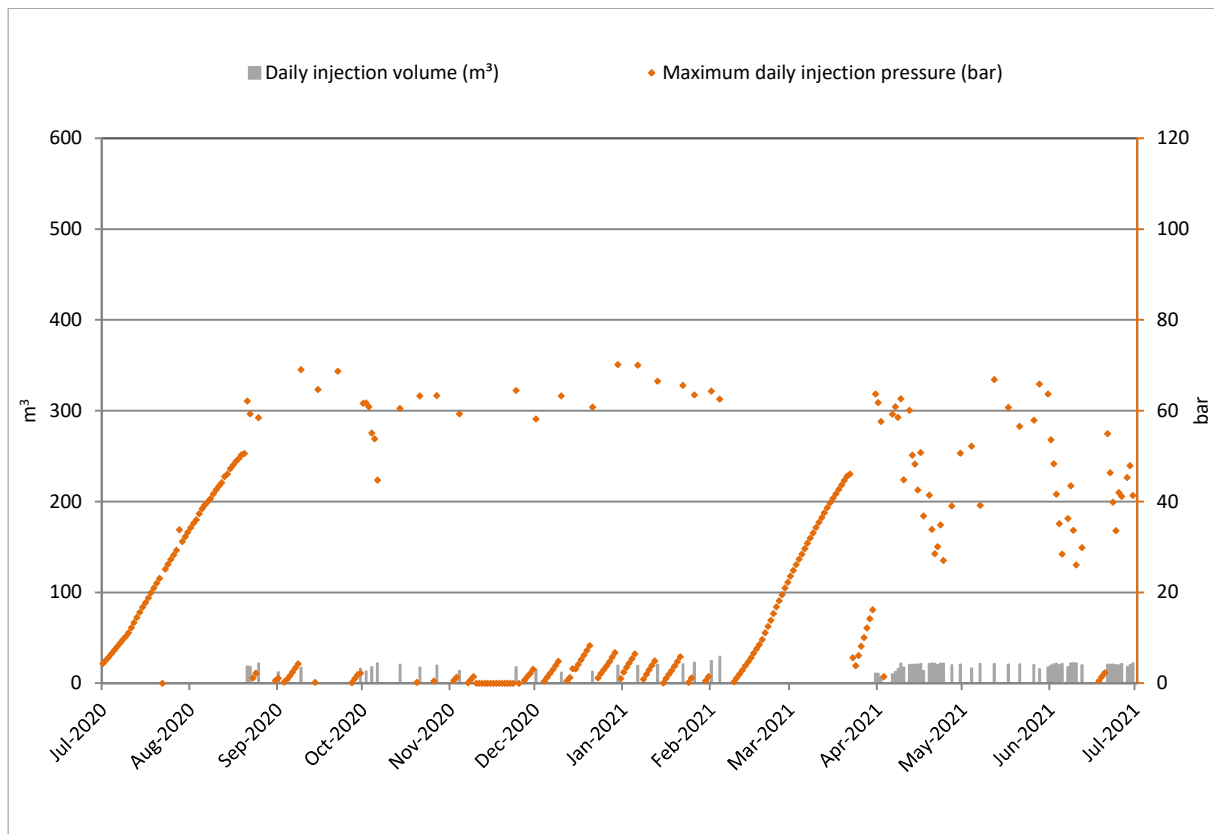
Figure 7 KA1/7/19/20 wellsite: KA1 well daily injection volume and pressure (2020-2021)
