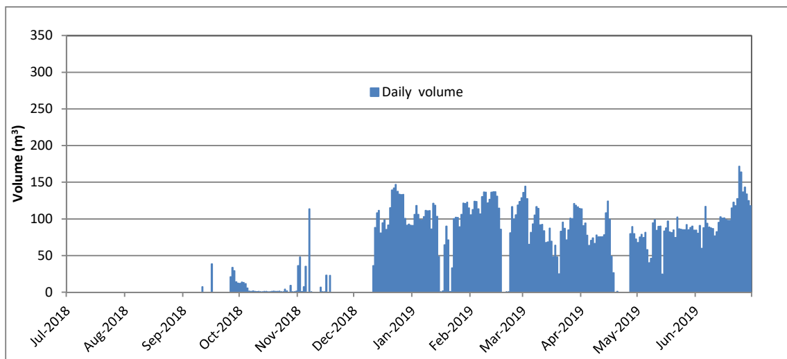
Figure 8 Manutahi-B2 well cumulative daily injection volumes (2018-2019)
