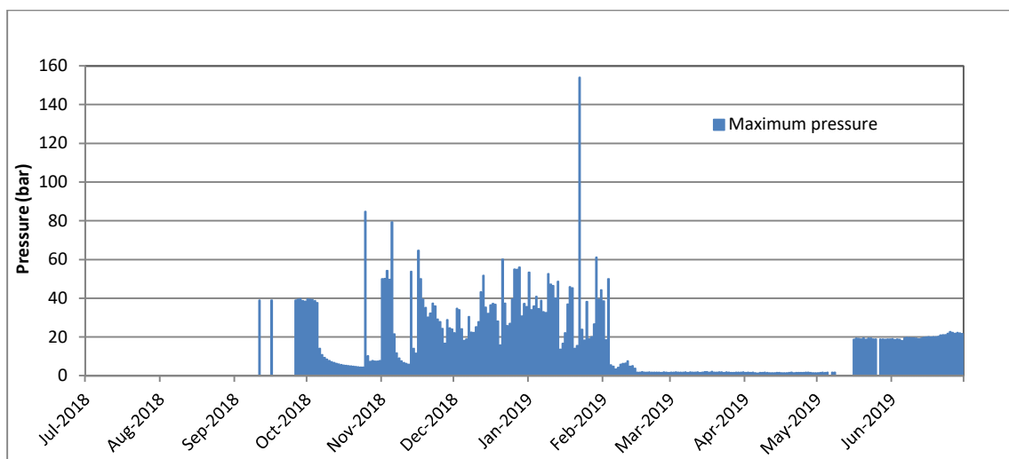
Figure 9 Manutahi-B2 upper daily maximum injection pressure (2018-2019)
