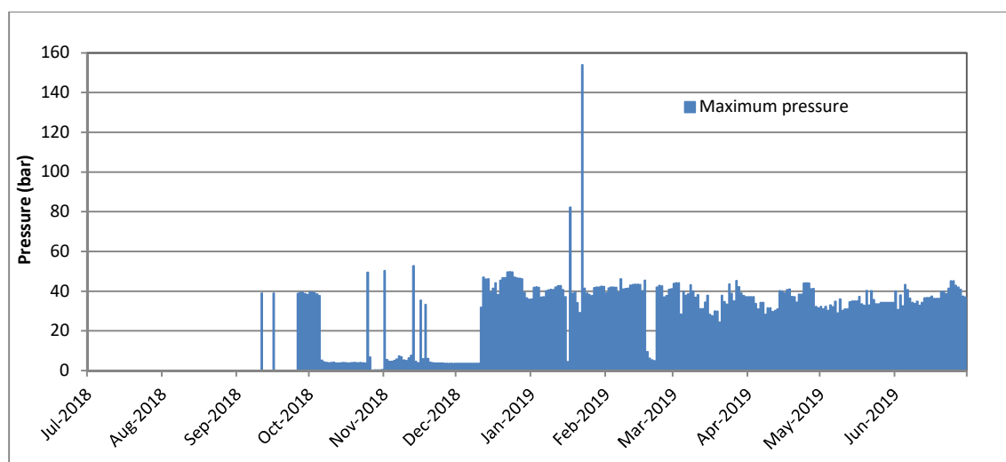
Figure 10 Manutahi-B2 lower daily maximum injection pressure (2018-2019)
