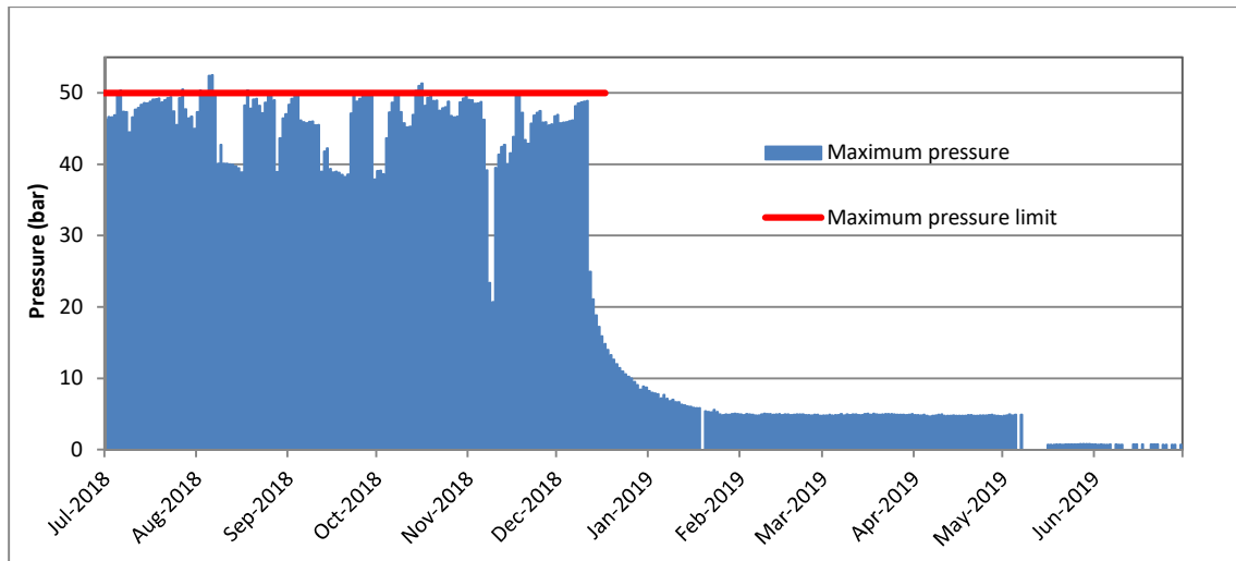
Figure 7 Manutahi-D4HST2 daily maximum injection pressure (2018-2019)
