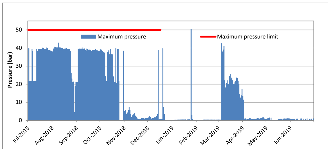
Figure 6 Manutahi-D2H daily maximum injection pressure (2018-2019)
