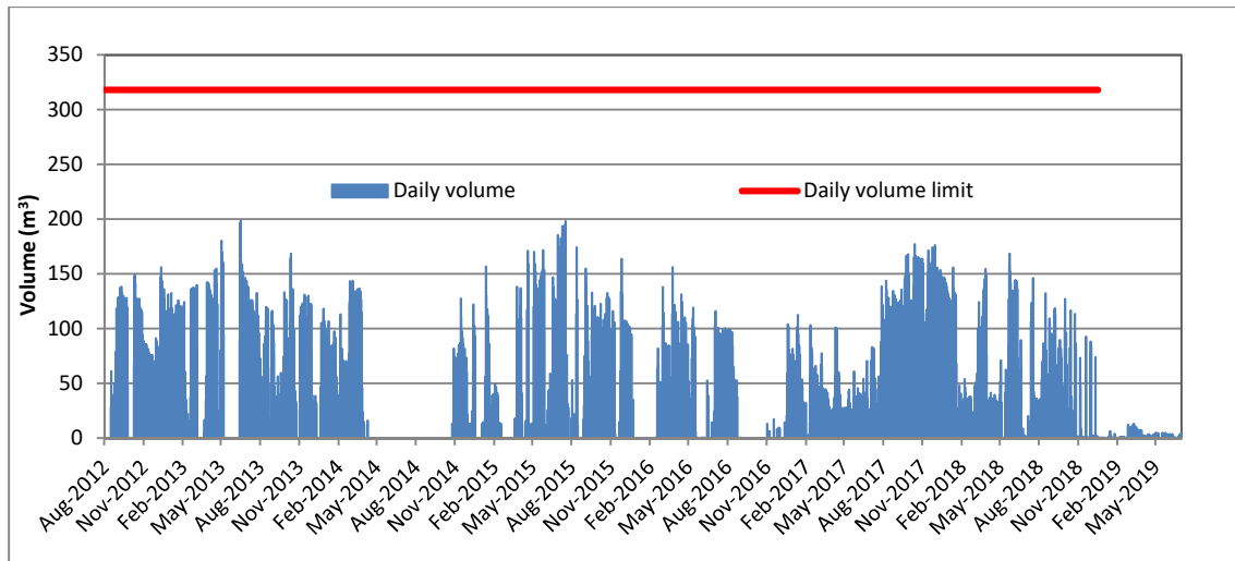
Figure 4 Manutahi-D cumulative daily injection volumes (2012-2019)
