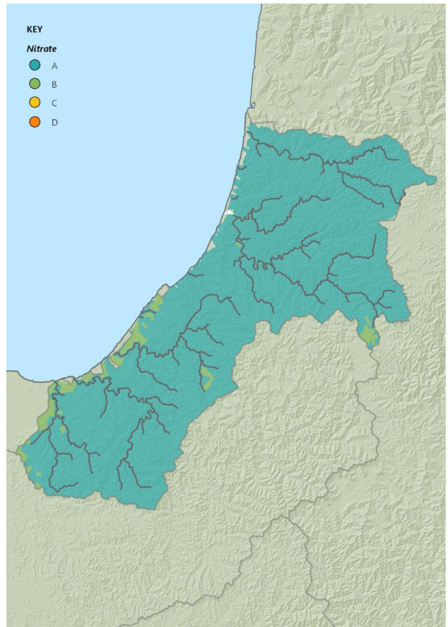
Figure 5 Nitrate modelling.
