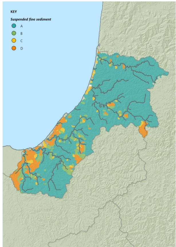
Figure 7 Suspended fine sediment modelling.
