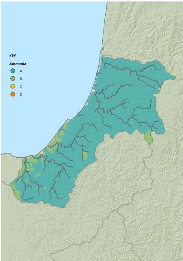
Figure 4 Ammonia modelling.
