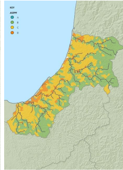
Figure 12 ASPM modelling.
