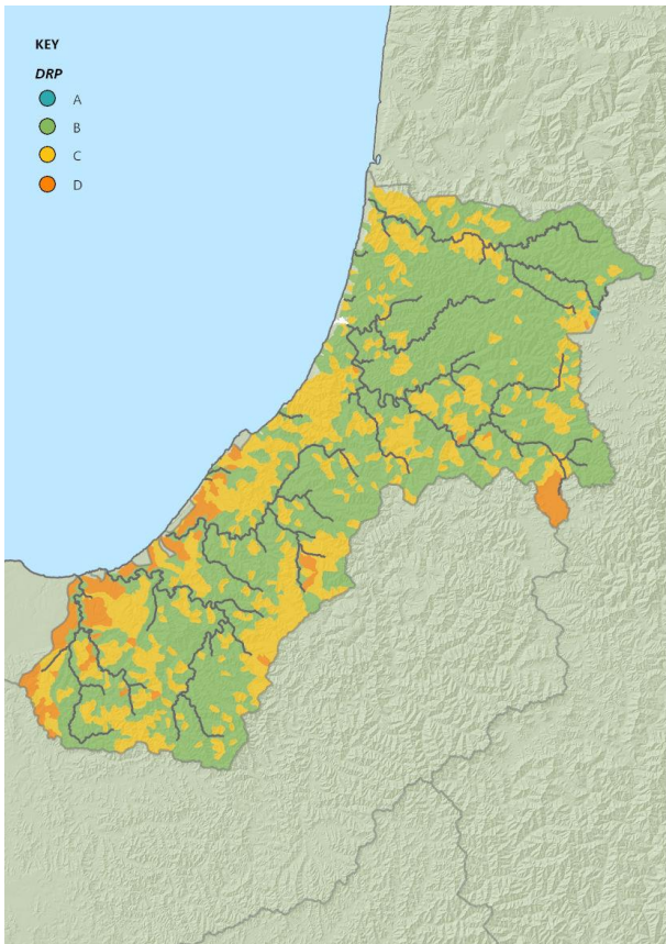
Figure 6 Dissolved reactive phosphorous modelling.
