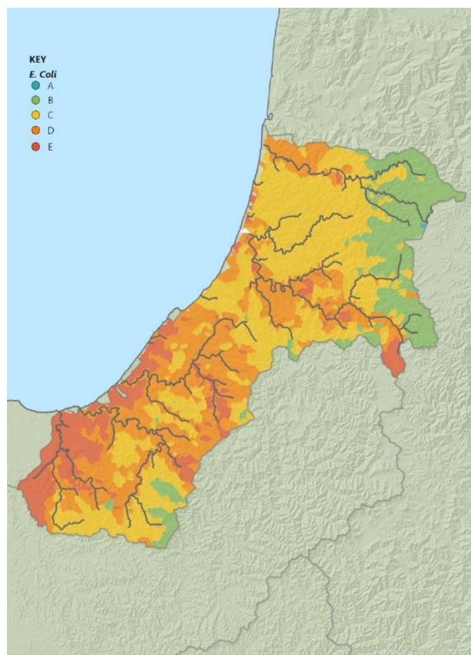
Figure 14 E. coli modelling (routine).
