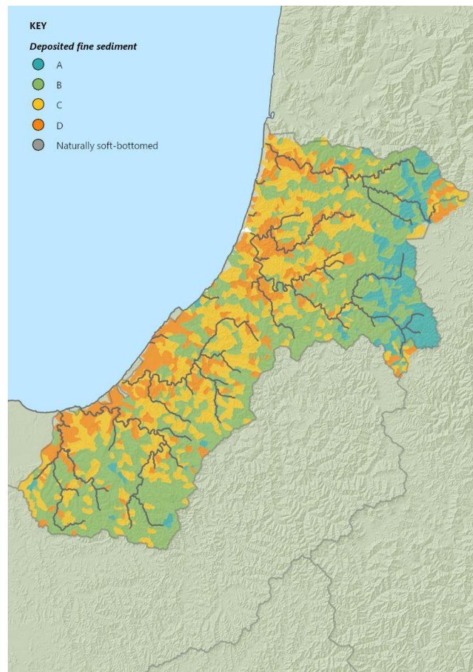
Figure 9 Deposited fine sediment modelling.
