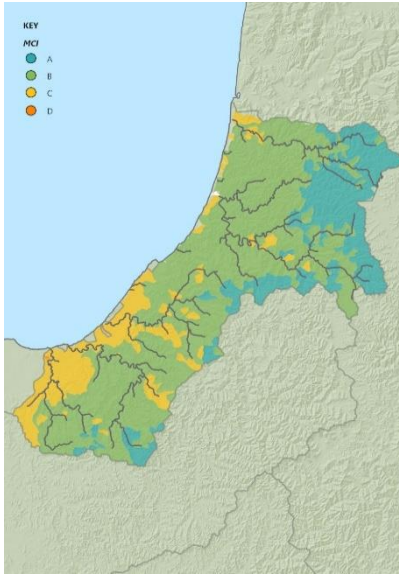
Figure 10 MCI modelling.
