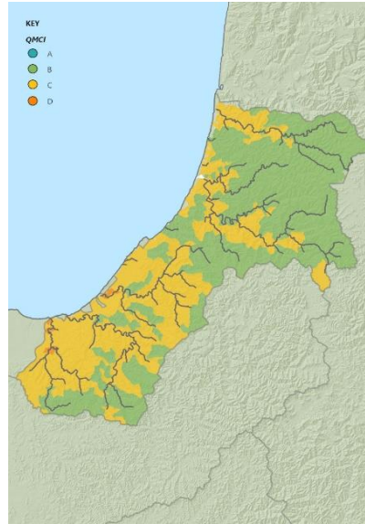
Figure 11 QMCI modelling.
