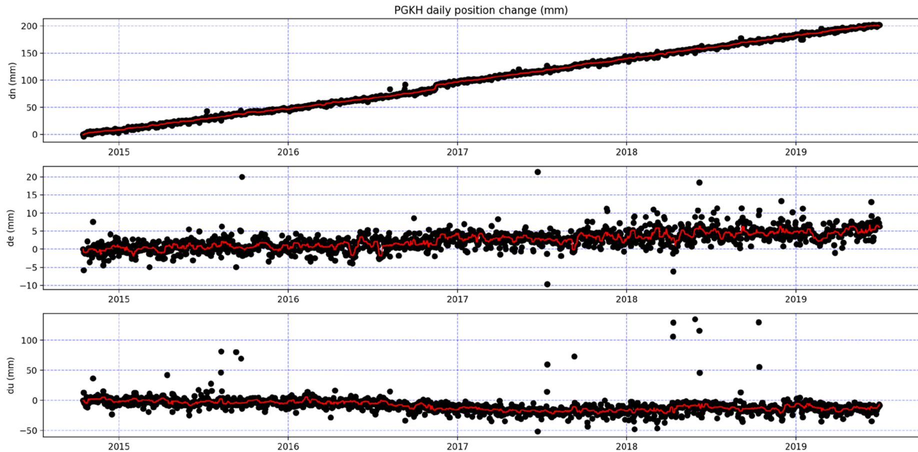
Figure 7.2 The displacement of the GNSS site PGKH at Kahui Hut on Mt Taranaki for 2014 to 2019. Displacements in the north-south (dn), east-west (de), and up-down (du) directions are shown. All positions are relative to the initial position when the sites were installed, and thus represent a displacement from the initial position. The black circles represent smoothed daily displacements. The red lines are the smoothed daily displacement curves. The Kaikōura earthquake occurred on 14 November 2016.
