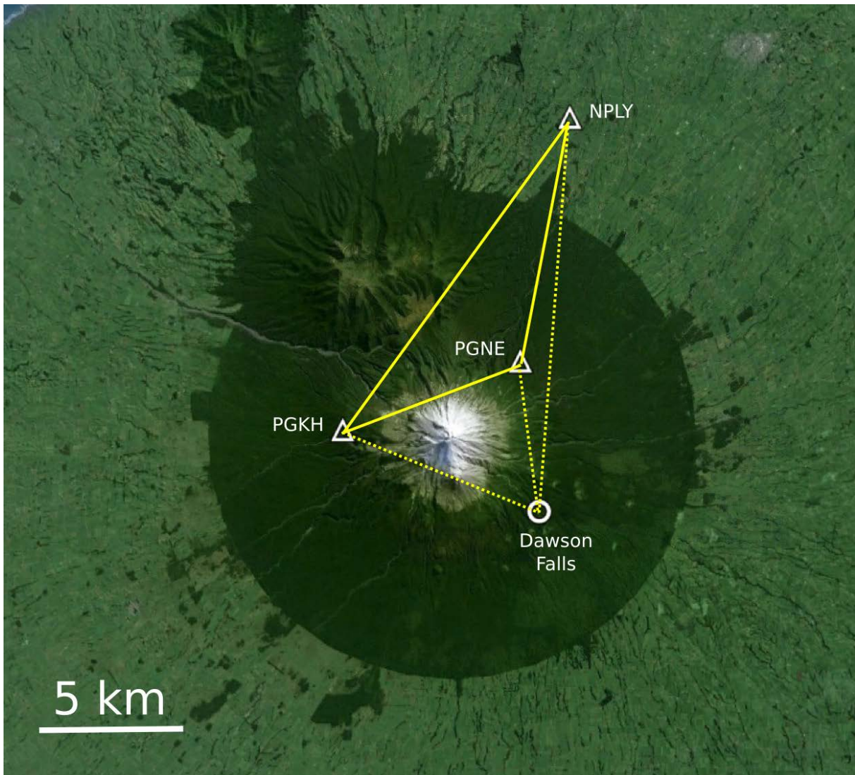
Figure 7.1 Locations of GeoNet GNSS sites on and near Mt Taranaki. Sites are labelled by their four-letter site codes. NPLY is New Plymouth (located on German Hill), PGKH is Kahui Hut and PGNE is North Egmont. The intention is to also install a site at Dawson Falls once redevelopment work planned in that area is completed by the Department of Conservation. Solid lines indicate line lengths currently able to be monitored. Dashed lines can be monitored when instruments are installed at Dawson Falls. The base map is from Google Earth.
