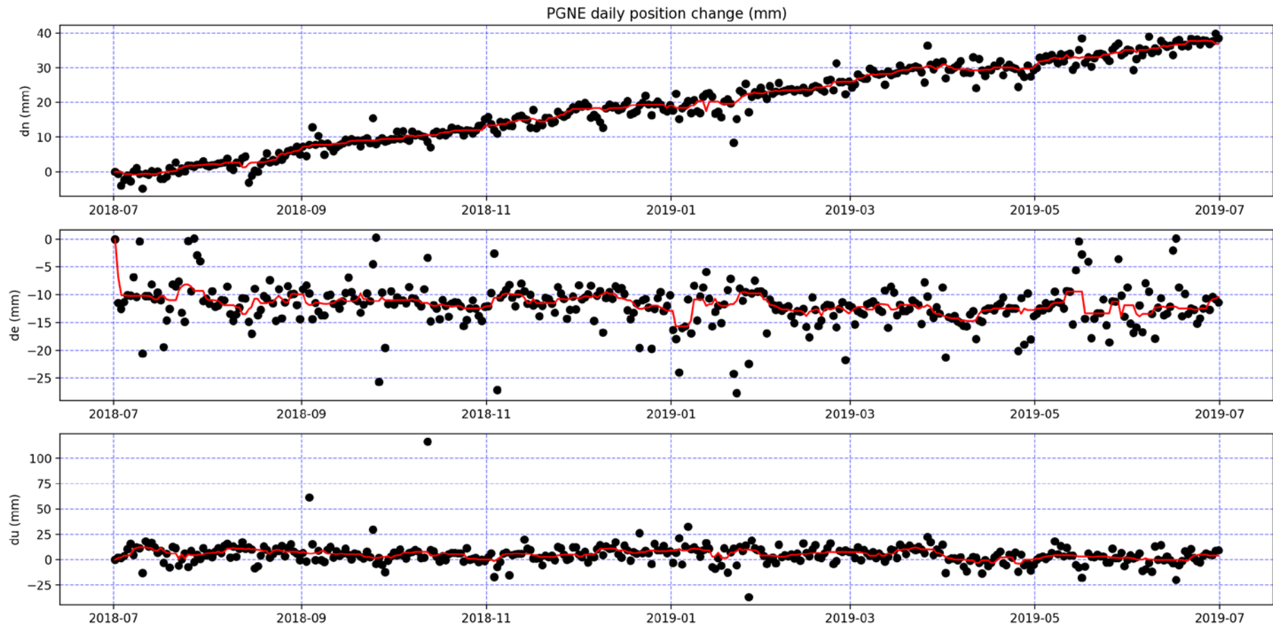
Figure 7.7 The displacement of the GNSS site PGNE at North Egmont on Mt Taranaki for 2018 to 2019. For further details refer to Figure 7.2.
