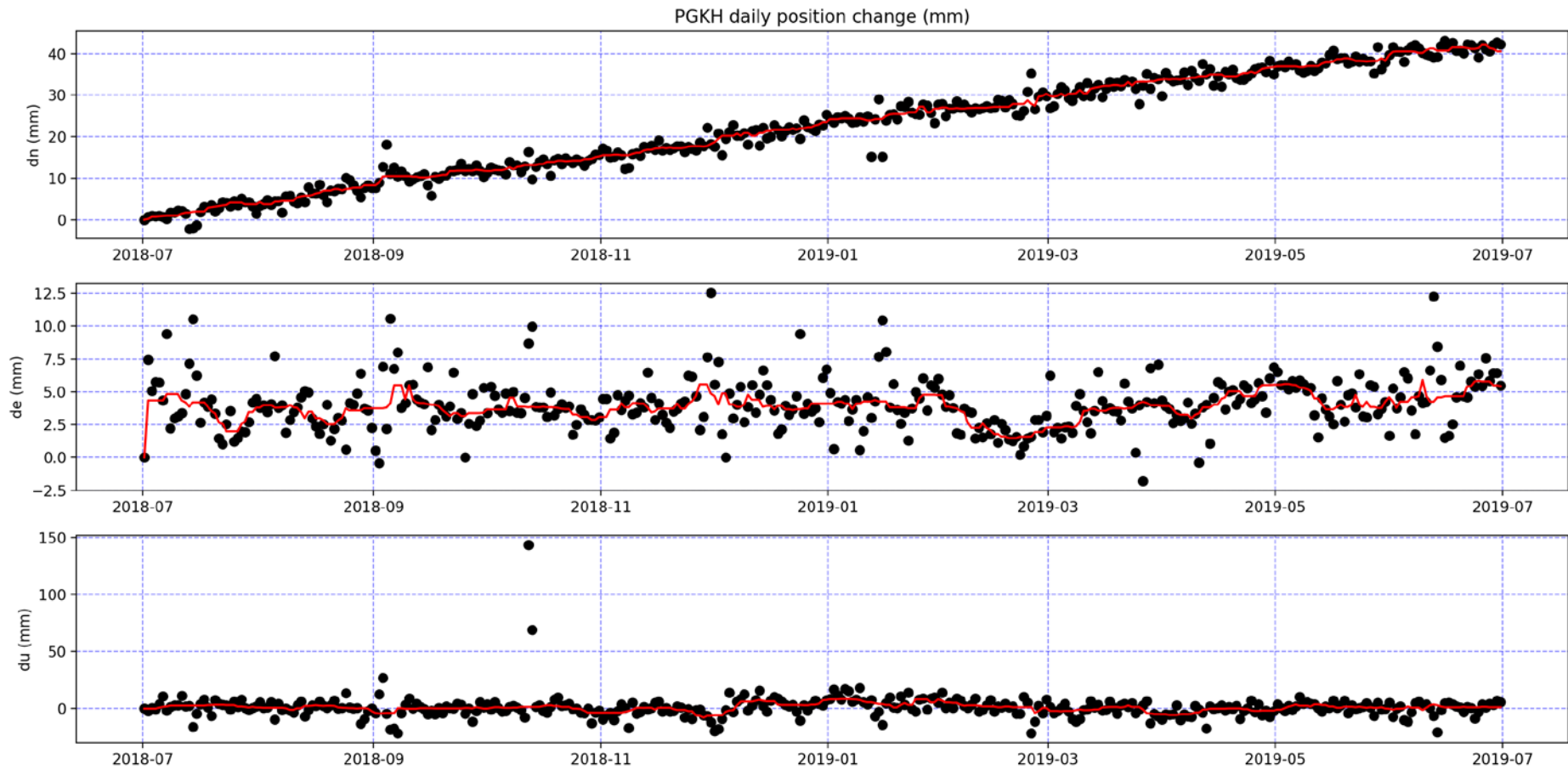
Figure 7.3 The displacement of the GNSS site PGKH at Kahui Hut on Mt Taranaki for 2018 to 2019. For further details refer to Figure 7.2.
