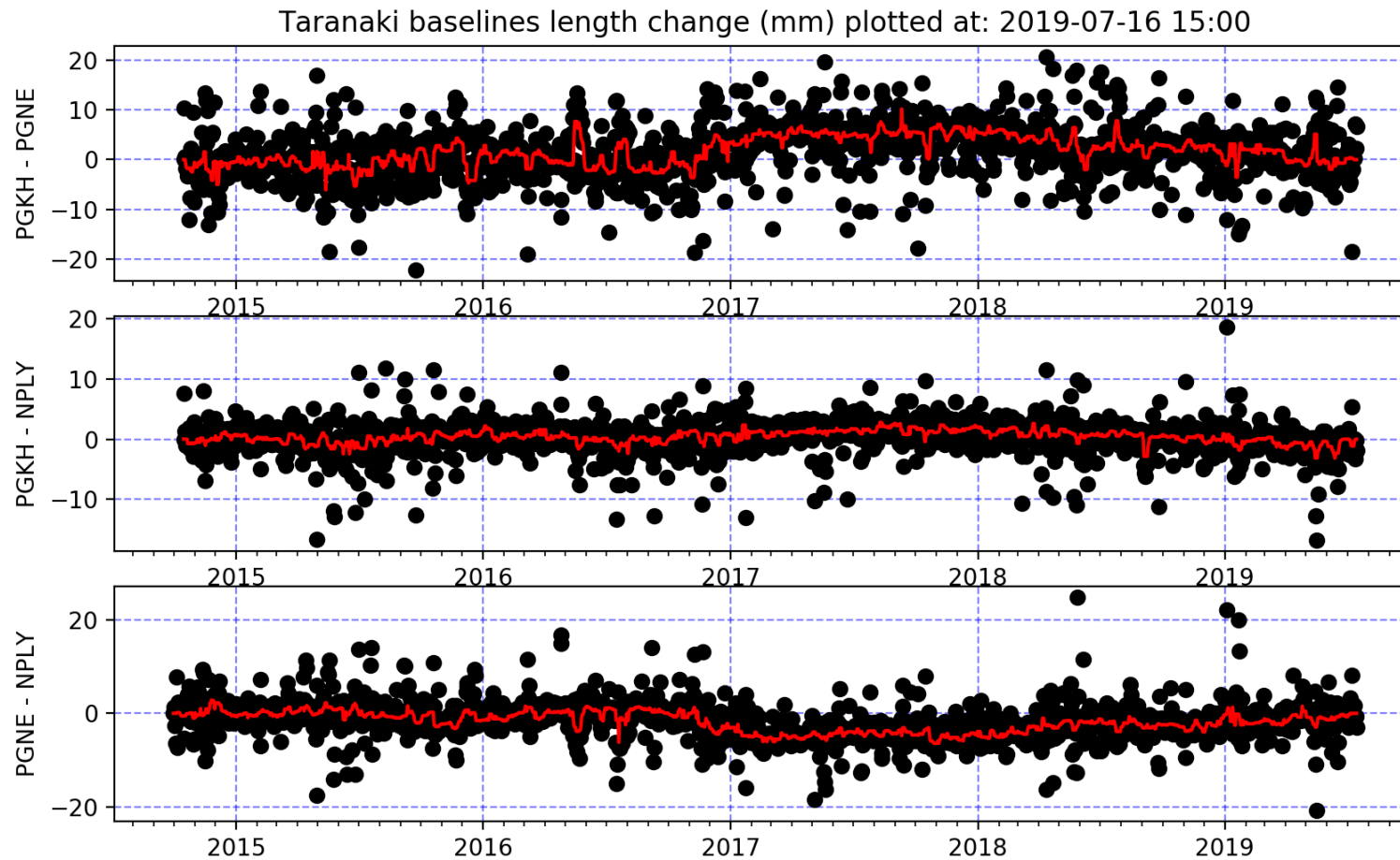
Figure 7.8 The length of lines between GNSS monitoring sites in Taranaki. The black circles represent daily line lengths and the red line a smoothed average. A slight change in the line lengths PGKH–PGNE and PGNE–NPLY is evident in late 2016. This occurred at the time of the 2016 November Kaikōura earthquake. It is not a result of locally sourced deformation but was caused by each of the GNSS sites responding slightly differently to that distant tectonic movement. Refer to Figures 7.1 and 7.2 for further details.
