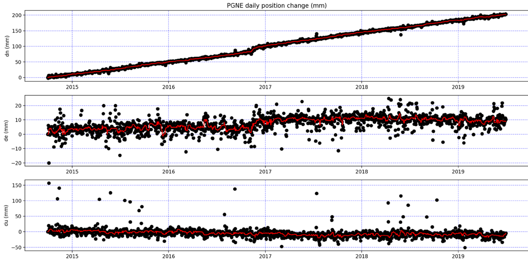
Figure 7.6 The displacement of the GNSS site PGNE at North Egmont on Mt Taranaki for 2014 to 2019. For further details refer to Figure 7.2.
