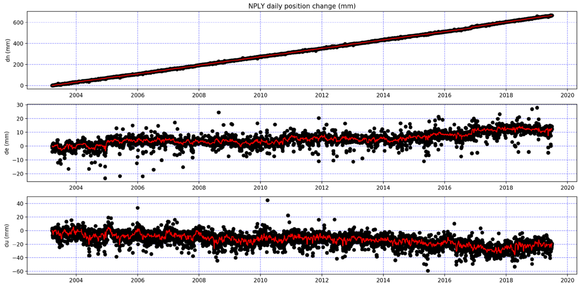
Figure 7.4 The displacement of the GNSS site NPLY at German Hill for 2003 to 2019. For further details refer to Figure 7.2.
