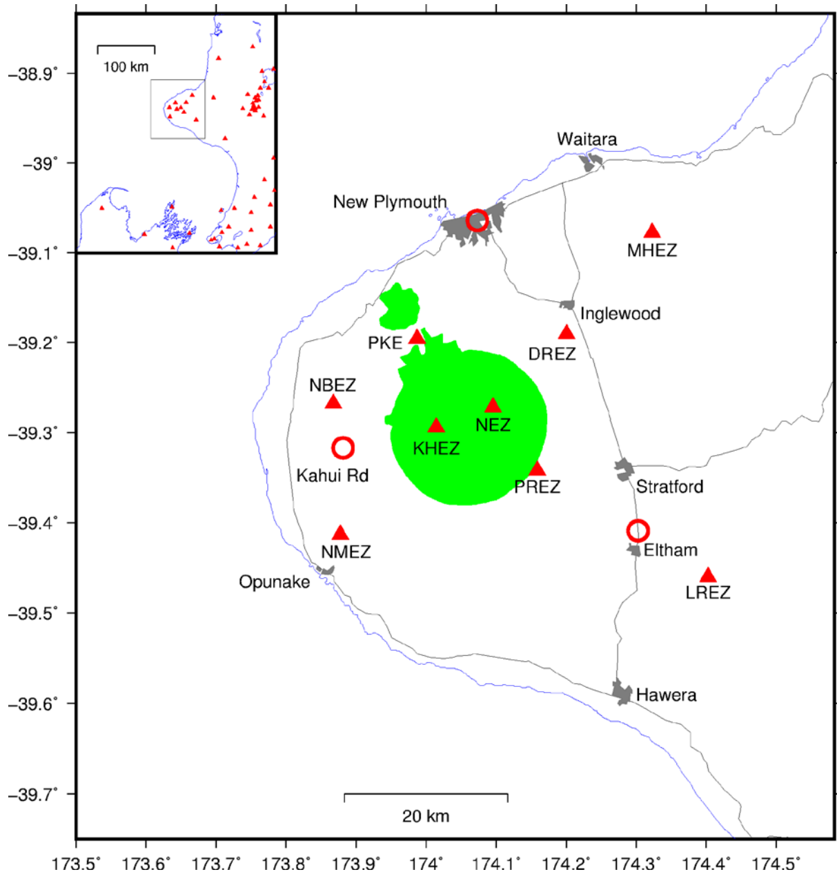
Figure 2.1 A map of the Taranaki seismographs as at 30 June 2019. Seismograph sites are indicated by red triangles and three or four-letter site codes. NEZ is North Egmont, NBEZ is Newall Road Borehole and PKE is Pukeiti. DREZ is Durham Road, MHEZ is Mangahewa and NMEZ is Namu Road. KHEZ is Kahui Hut, PREZ is Palmer Road and LREZ is Lake Rotokare. Data connection (hub) sites are shown by red circles. Main population centres are shown in grey and named. The Egmont National Park is shown as a green area. Major roads are shown as black lines. The coastline is marked in blue. The inset shows Taranaki and nearby GeoNet seismographs (red triangles), some of which are used in locating earthquakes in the Taranaki region.
